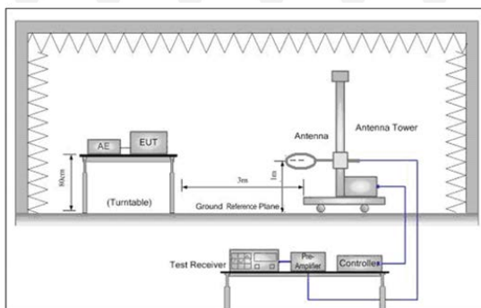
Figure 1. Below 30MHz
