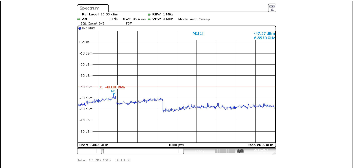
Band40-5MHz-QPSK-39225-1RB#0-Range13:2365~26500MHz
