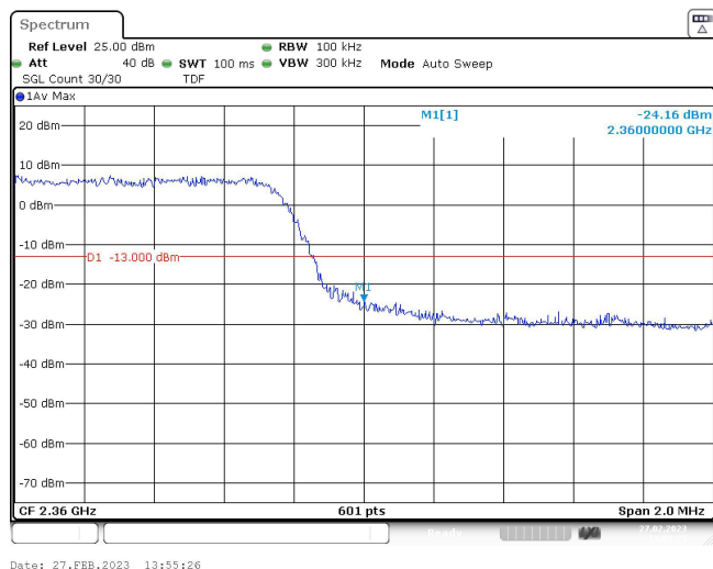
Band40-5MHz-16QAM-39175-1RB#0
