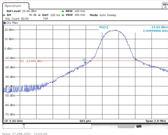
Band40-5MHz-16QAM-39175-1RB#24
