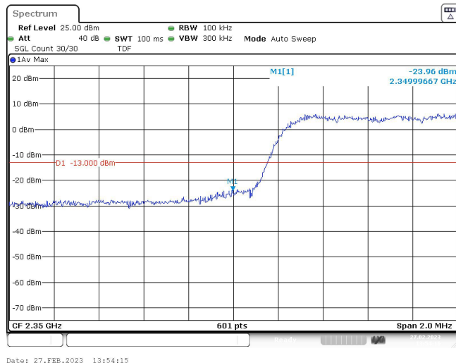
Band40-5MHz-16QAM-39225-1RB#0
