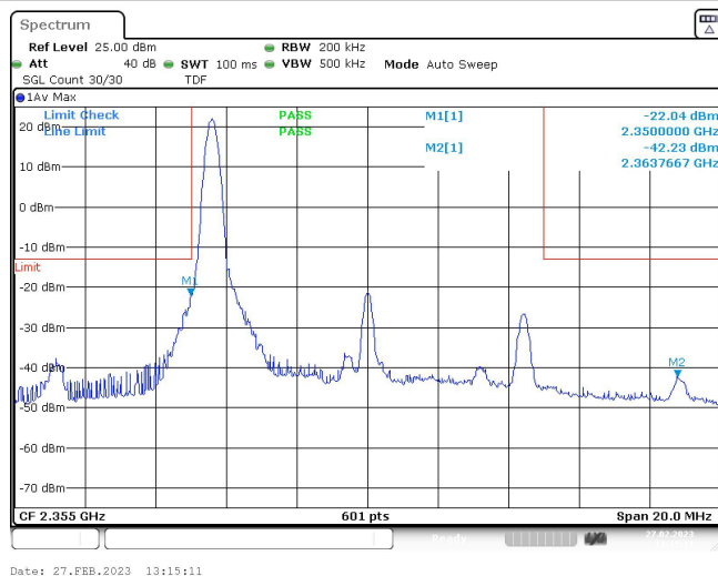
Band40-10MHz-QPSK-39200-1RB#49
