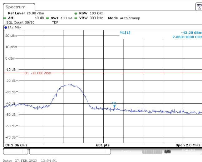
Band40-5MHz-16QAM-39225-1RB#24
