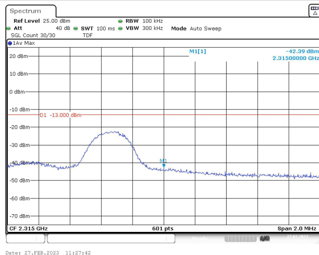
Band40-5MHz-QPSK-38775-1RB#24
