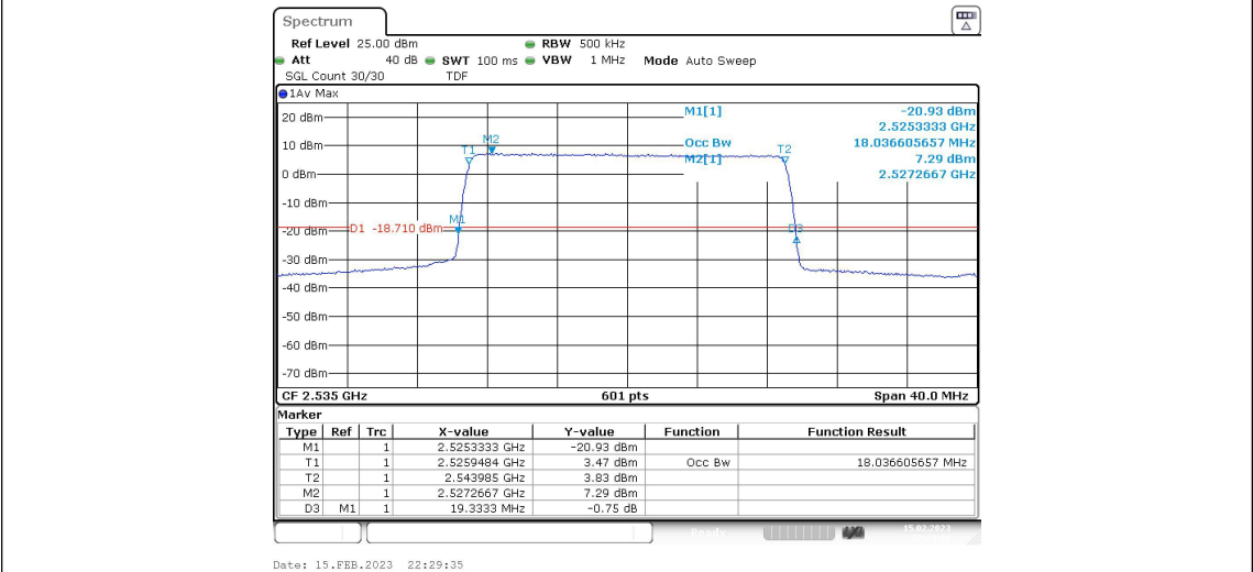
Band7-20MHz-QPSK-21350-100RB#0
