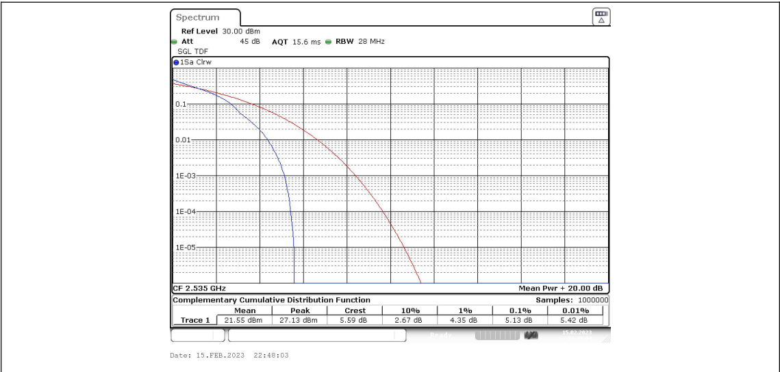
Band7-20MHz-QPSK-21100-100RB#0
