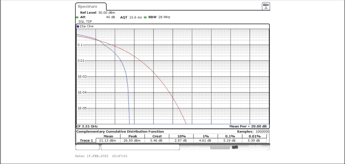
Band7-20MHz-16QAM-20850-100RB#0
