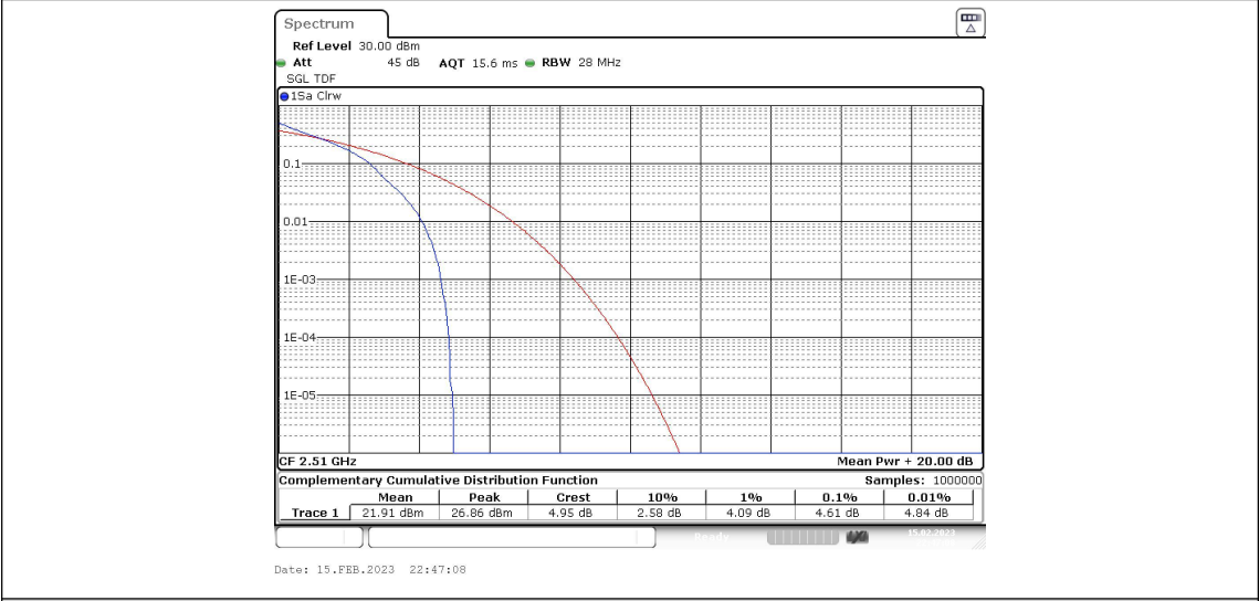
Band7-20MHz-QPSK-20850-100RB#0
