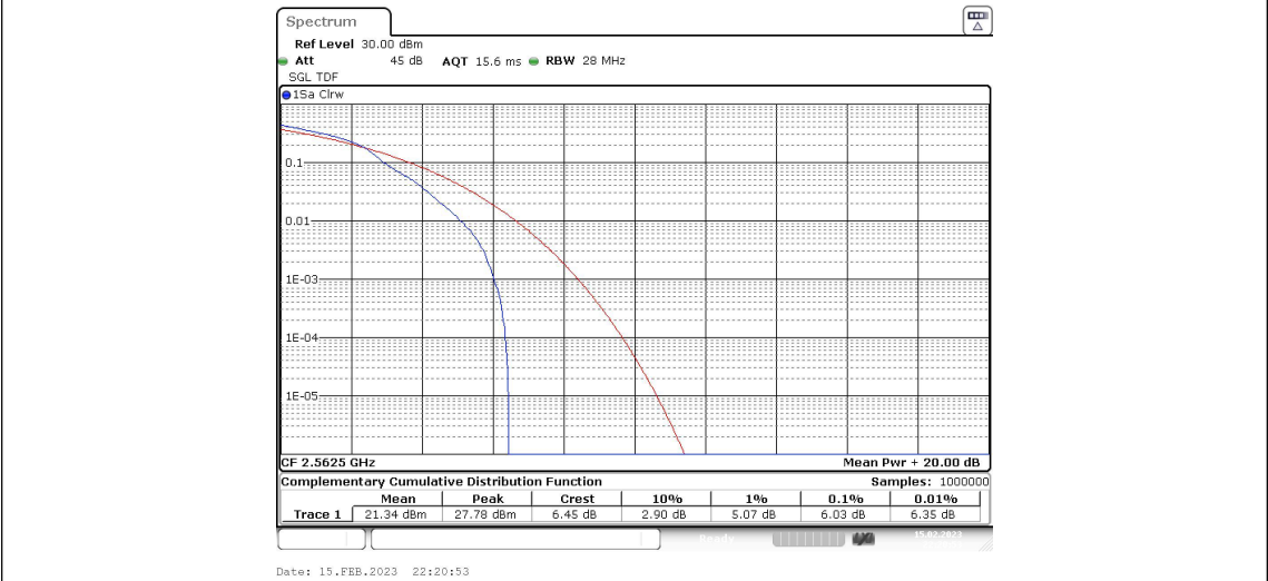
Band7-15MHz-16QAM-21375-75RB#0
