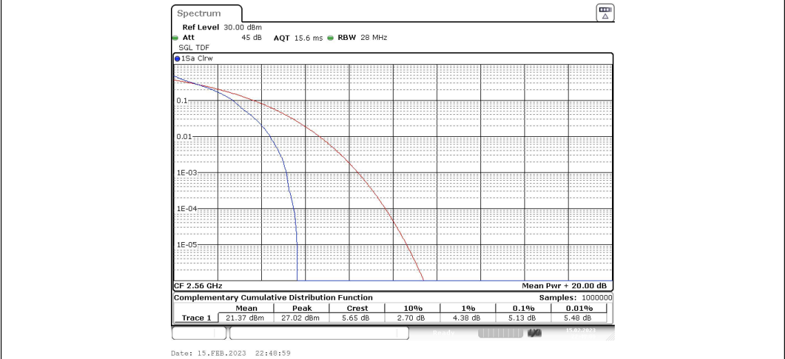
Band7-20MHz-QPSK-21350-100RB#0
