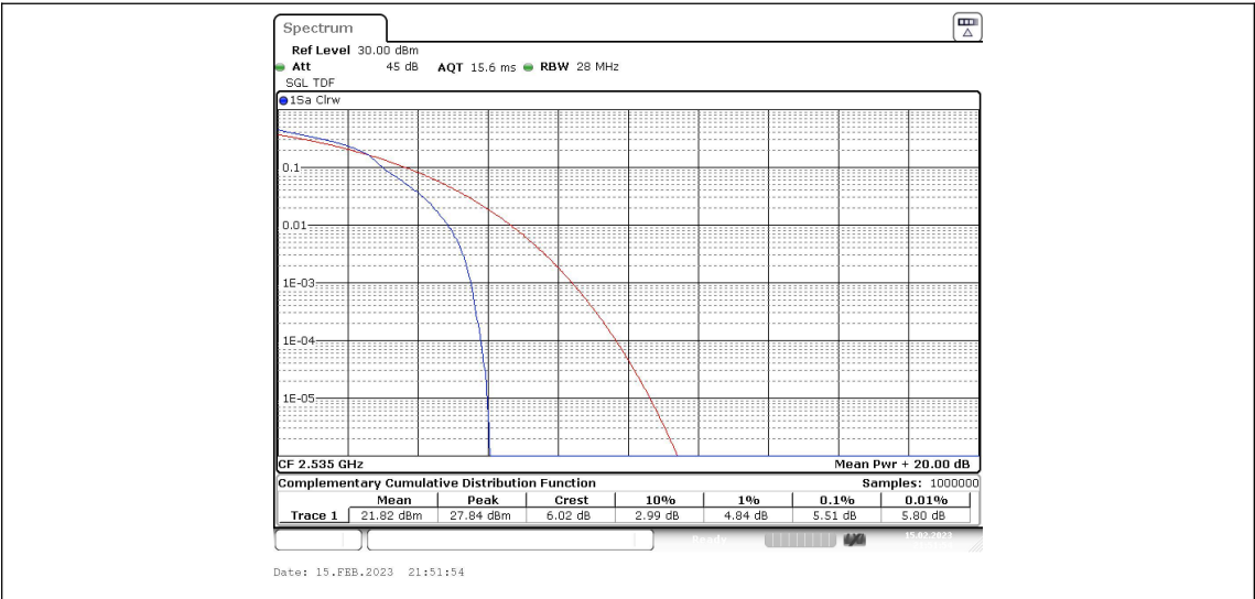
Band7-10MHz-16QAM-21100-50RB#0
