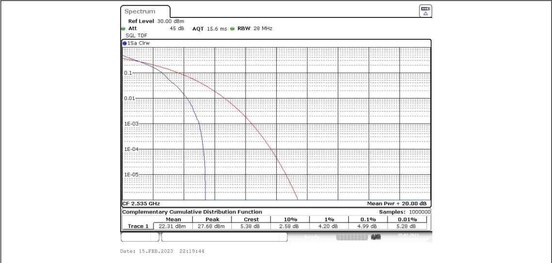
Band7-15MHz-QPSK-21100-75RB#0
