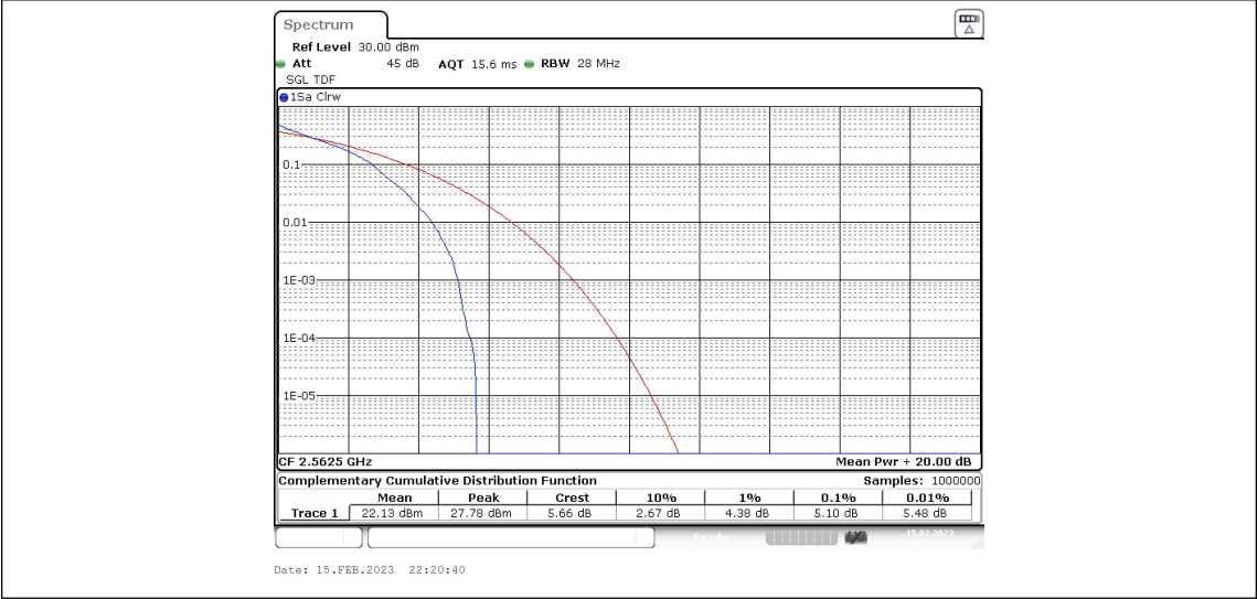
Band7-15MHz-QPSK-21375-75RB#0
