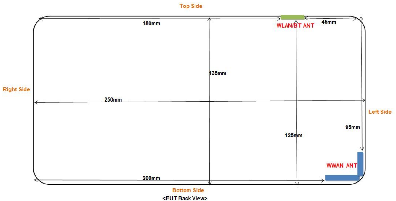
Block Diagram for EUT Antenna Position
