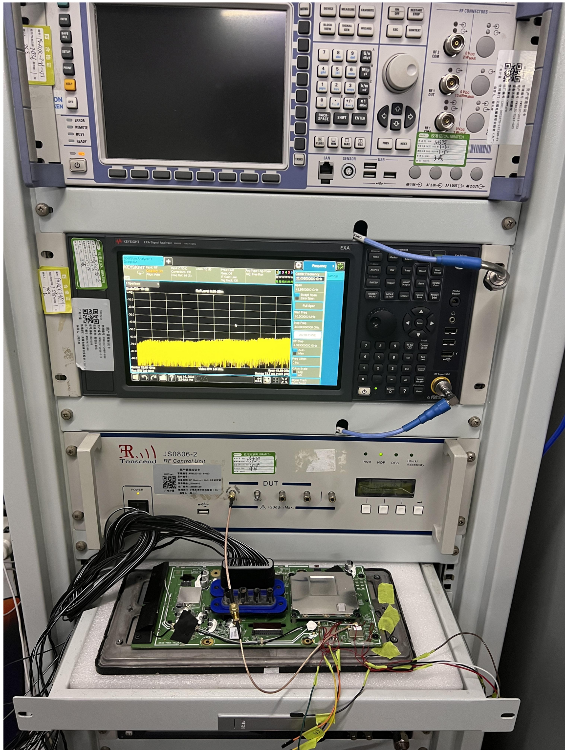
Description: Conducted Test Setup Photo
