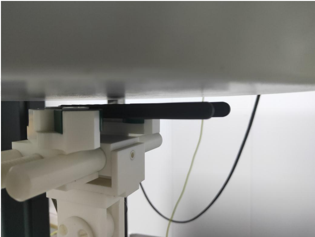
5mm body Horizontal-Up Side Setup Photo – Test Position 2
