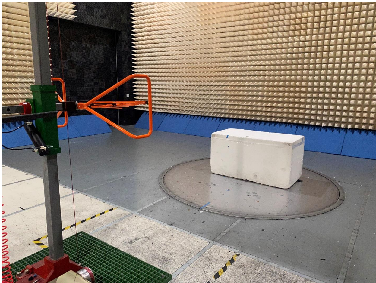
Figure 2: FCC 15.247 RSE, 30MHz – 1GHz
