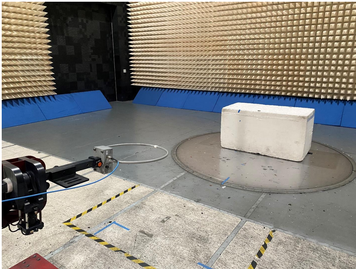
Figure 1: FCC 15.247 RSE, 9kHz – 30MHz
