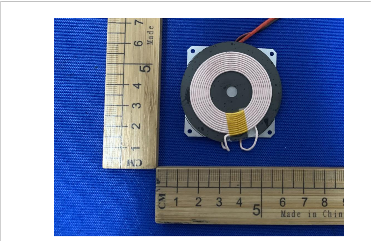
Details of: Internal view for model DK-WL-001, DK-WL-002
