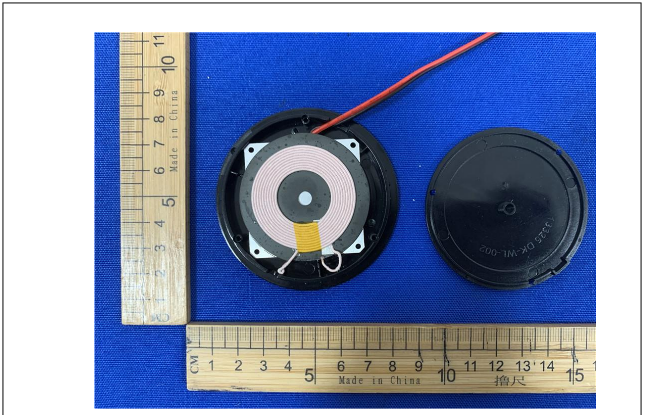
Details of: Internal view for model DK-WL-002
