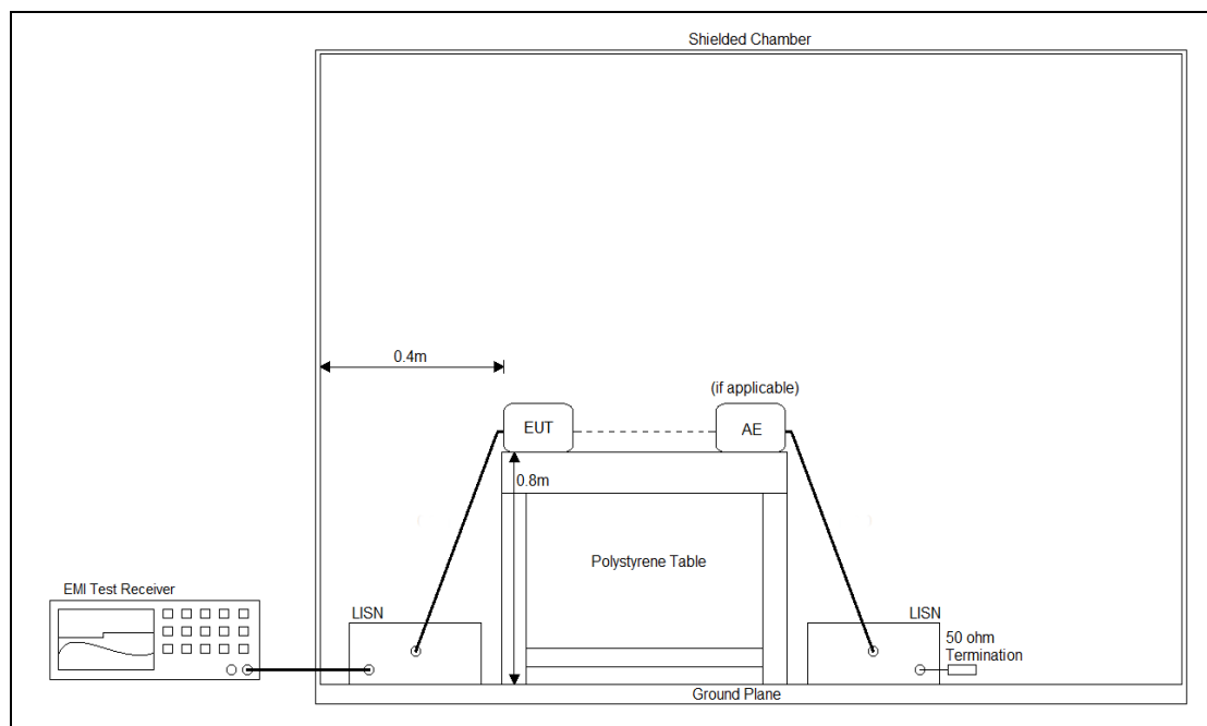
Figure 3: Test setup
