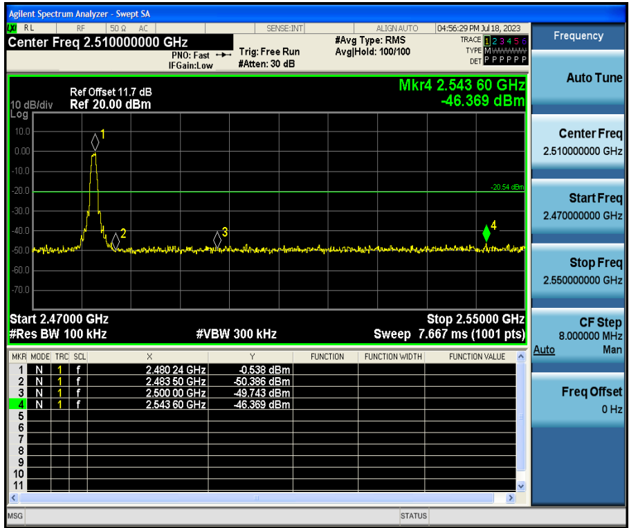
BLE_1M-Ant1-2480
