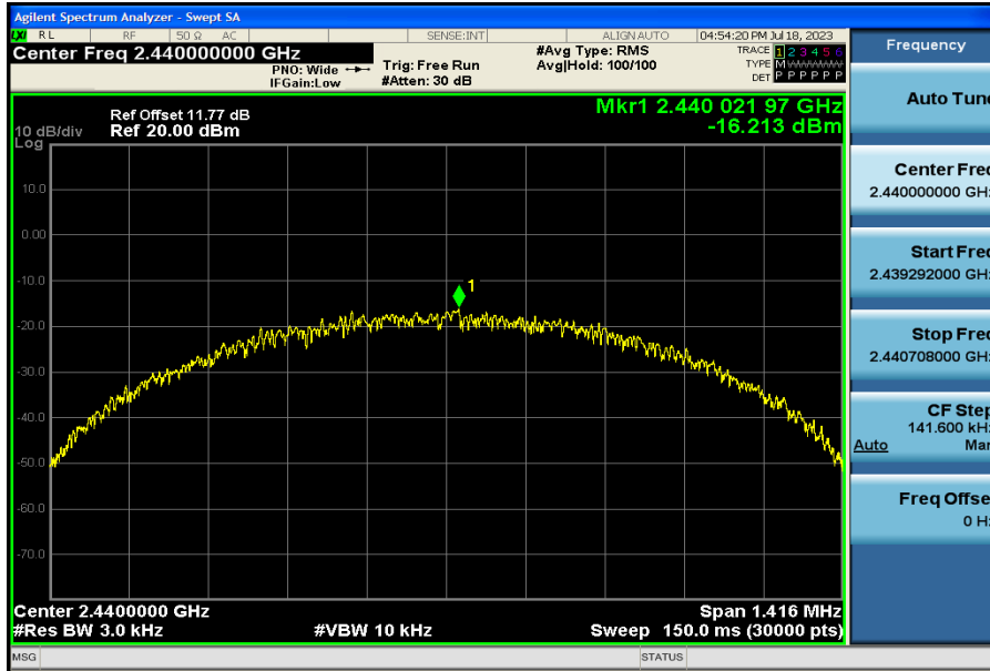
BLE_1M-Ant1-2440
