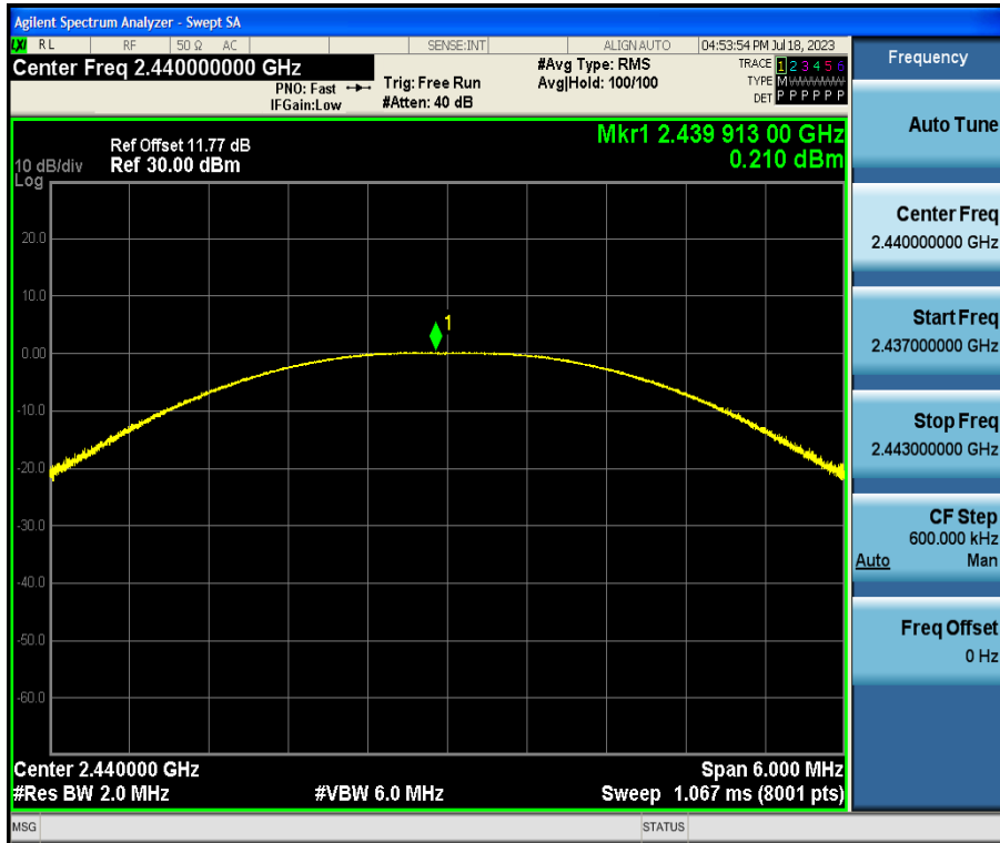
BLE_1M-Ant1-2440
