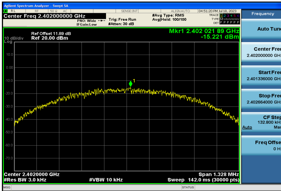
BLE_1M-Ant1-2402
