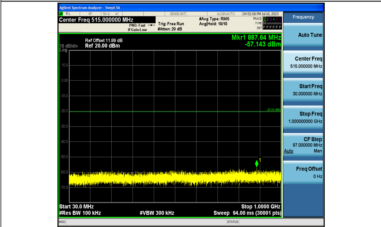
BLE_1M-Ant1-2402-0~Reference
