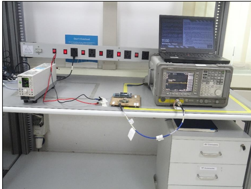
Antenna Port Measurement Test Setup
