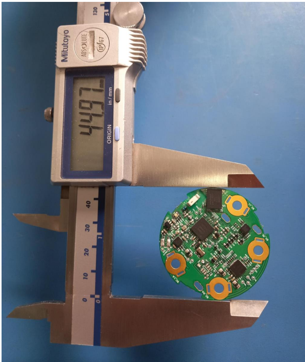
PCB Dimensional View
