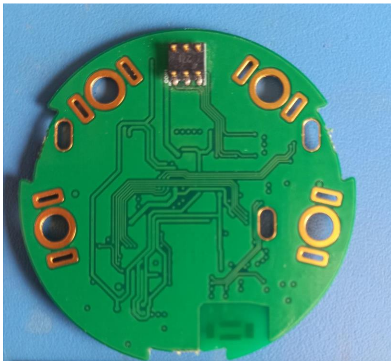
PCB_Rear View
