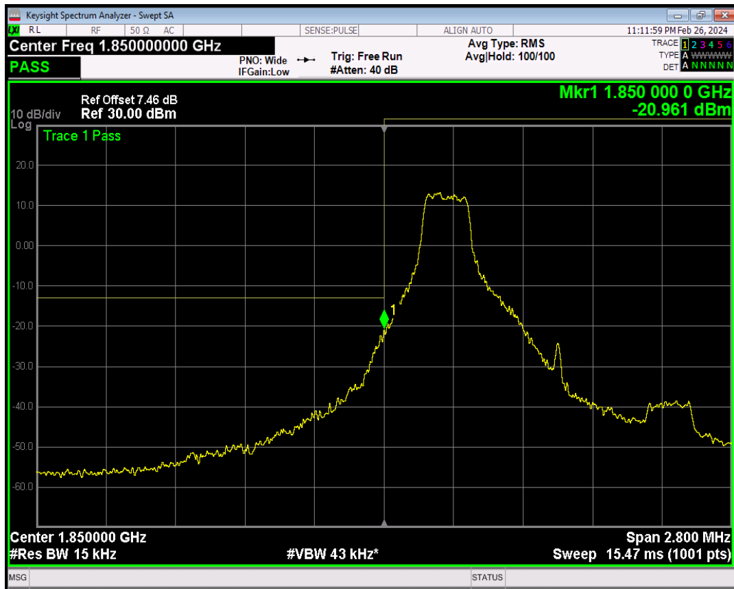
Band25 16QAM BW=1.4MHz Channel=26047 RB Size=1 Position=#Max
