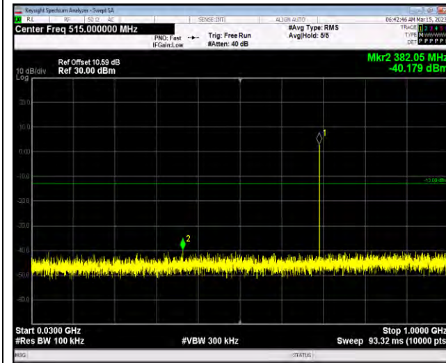
Band12-1.4MHz-64QAM-23095-1RB#0-Range1:30 ~1000MHz
