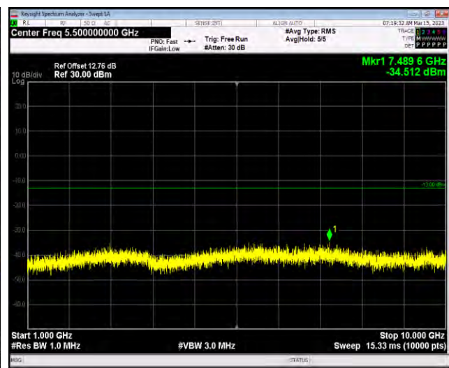
Band12-10MHz-64QAM-23130-1RB#0-Range2:1000~ 10000MHz
