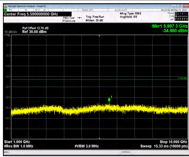
Band12-1.4MHz-64QAM-23095-1RB#0-Range2:1000 ~10000MHz
