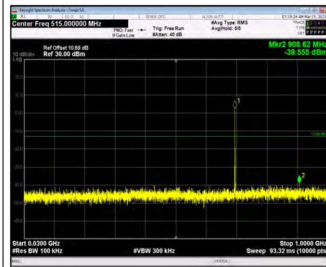
Band12-10MHz-64QAM-23130-1RB#0-Range1:30 ~1000MHz
