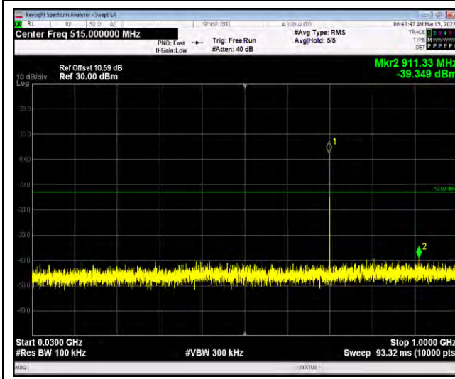
Band12-1.4MHz-64QAM-23095-1RB#0-Range1:30 ~1000MHz
