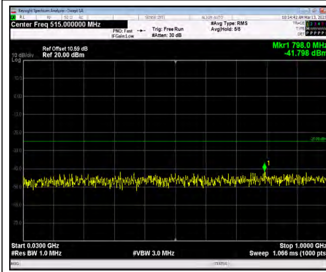
Band7-20MHz-64QAM-20850-1RB#0-Range1:30~1000MHz
