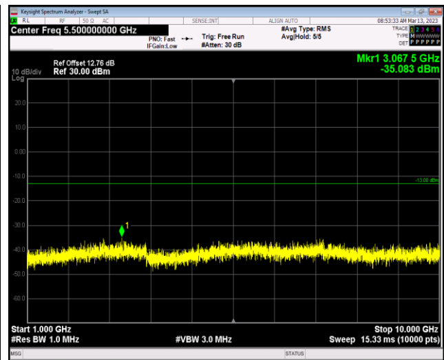
Band5-1.4MHz-16QAM-20643-1RB#0-Range2:1000~10000MHz
