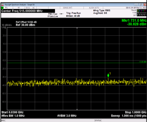
Band4-20MHz-16QAM-20300-1RB#0-Range1:30~ 1000MHz
