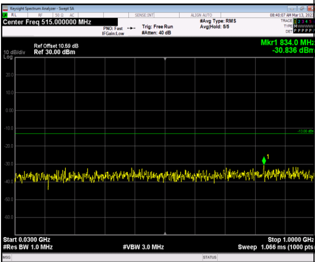
Band4-20MHz-16QAM-20175-1RB#0-Range1:30~ 1000MHz
