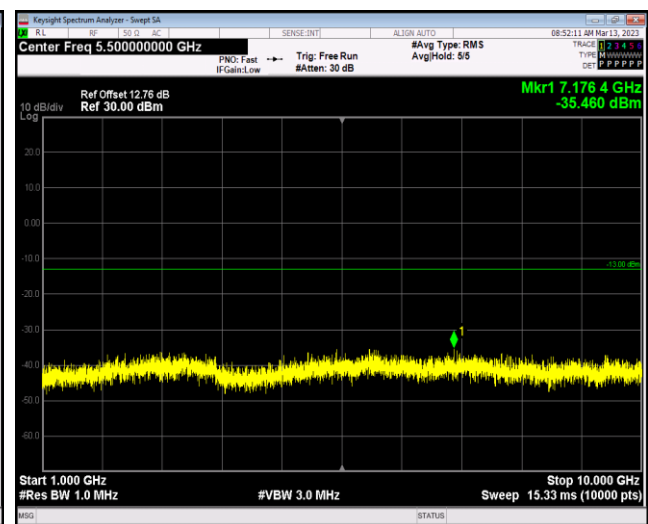
Band5-1.4MHz-QPSK-20525-1RB#0-Range2:1000~10000MHz
