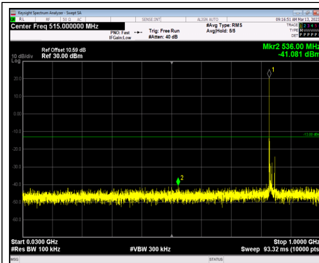
Band5-10MHz-64QAM-20600-1RB#0-Range1:30~1000MHz
