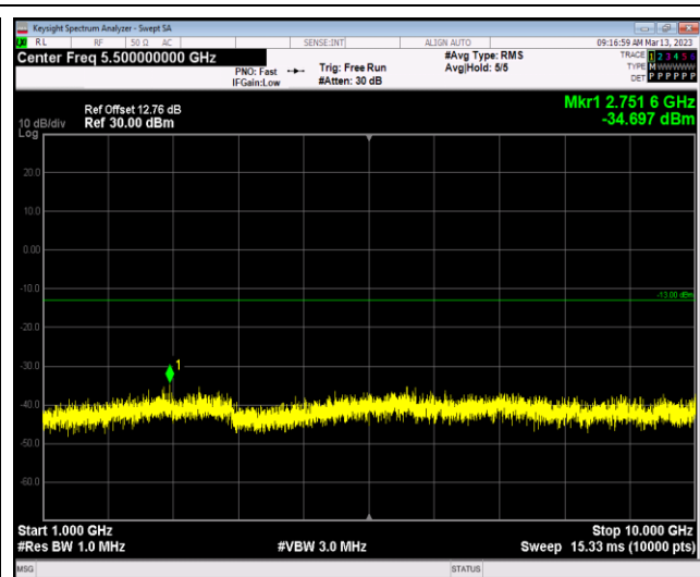
Band5-10MHz-64QAM-20600-1RB#0-Range2:1000~10000MHz
