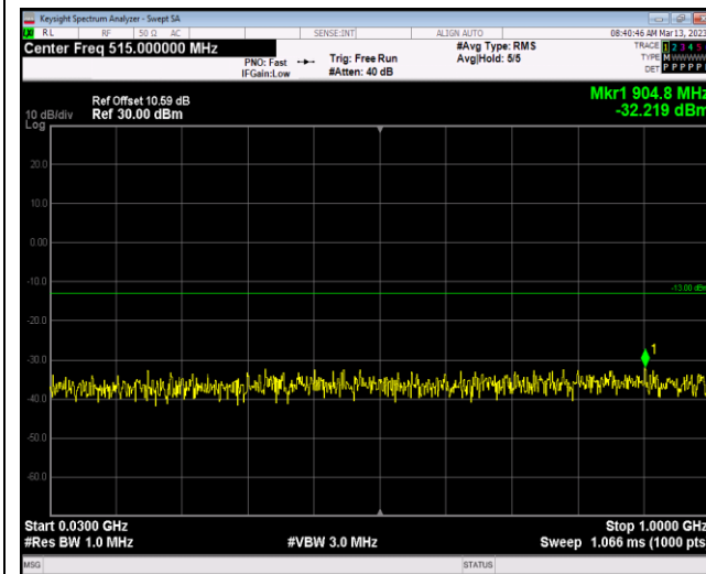
Band4-20MHz-QPSK-20300-1RB#0-Range1:30~1000MHz
