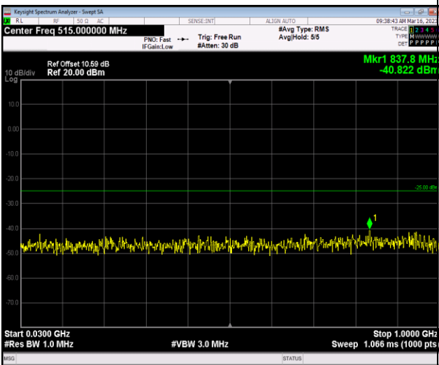
Band7-5MHz-64QAM-21100-1RB#0-Range1:30~1 000MHz
