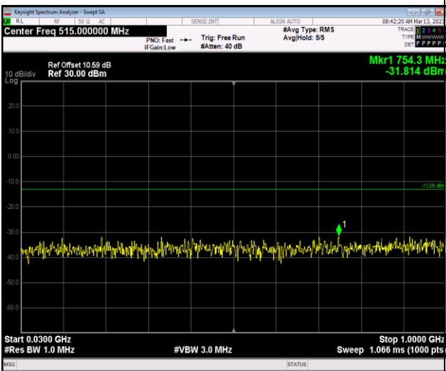
Band5-1.4MHz-QPSK-20407-1RB#0-Range1:30~1000MHz
