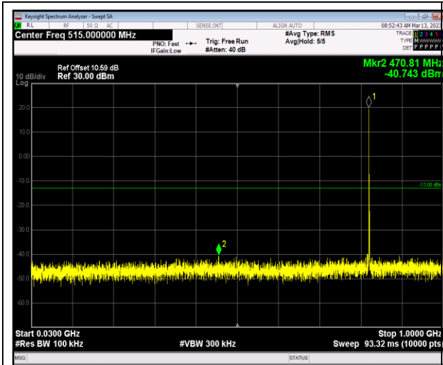
Band5-1.4MHz-64QAM-20525-1RB#0-Range1:30~1000MHz
