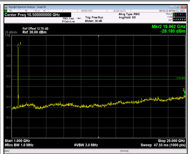
Band4-20MHz-64QAM-20050-1RB#0-Range2:1000~20000MHz
