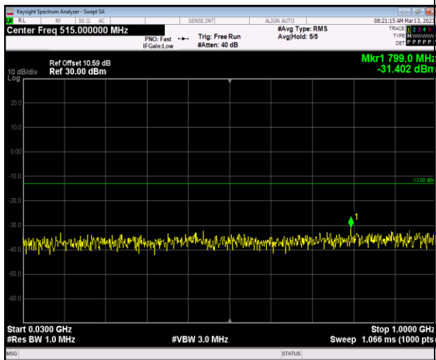
Band4-1.4MHz-64QAM-20393-1RB#0-Range1:30~ 1000MHz
