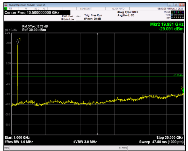
Band4-20MHz-64QAM-20175-1RB#0-Range2:1000~20000MHz
