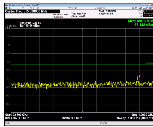
Band4-1.4MHz-64QAM-19957-1RB#0-Range1:30~1000MHz
