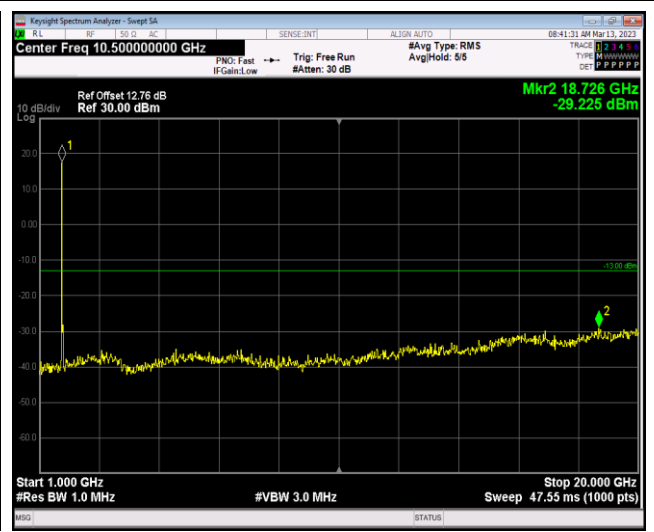
Band4-20MHz-64QAM-20175-1RB#0-Range2:1000~20000MHz
