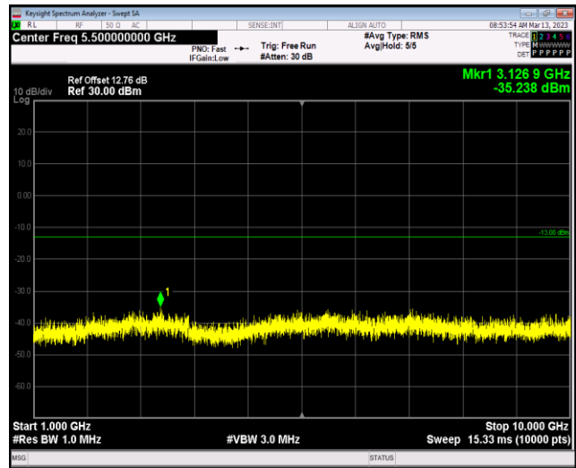
Band5-1.4MHz-64QAM-20643-1RB#0-Range2:1000~10000MHz
