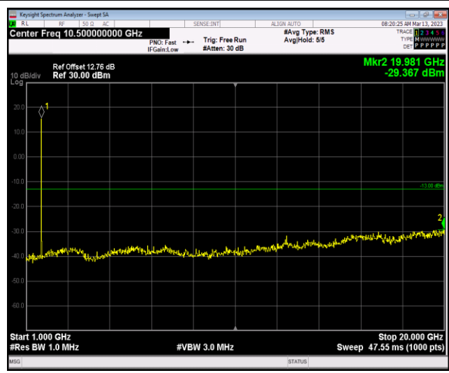
Band4-1.4MHz-64QAM-19957-1RB#0-Range2:1000~20000MHz
