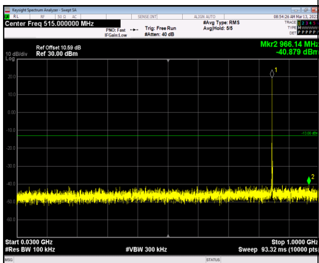
Band5-1.4MHz-64QAM-20407-1RB#0-Range1:30~1000MHz
