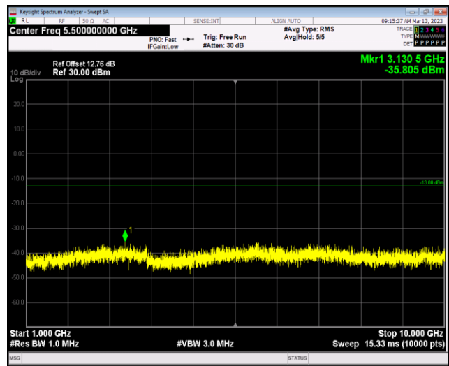
Band5-10MHz-16QAM-20525-1RB#0-Range2:1000~10000MHz
