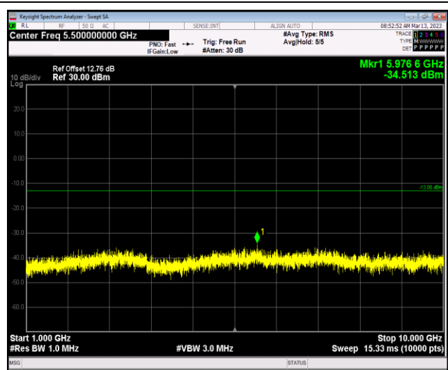
Band5-1.4MHz-64QAM-20525-1RB#0-Range2:1000~10000MHz
