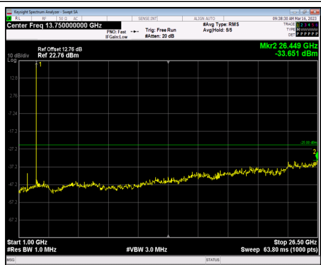
Band7-5MHz-16QAM-21100-1RB#0-Range2:1000~26 500MHz
