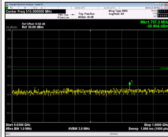
Band4-20MHz-64QAM-20175-1RB#0-Range1:30~1000MHz
