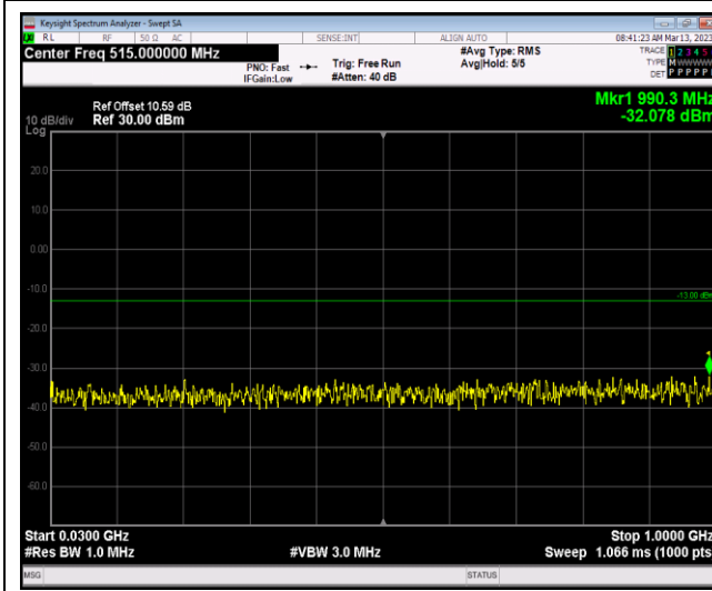
Band4-20MHz-64QAM-20175-1RB#0-Range1:30~1000MHz
