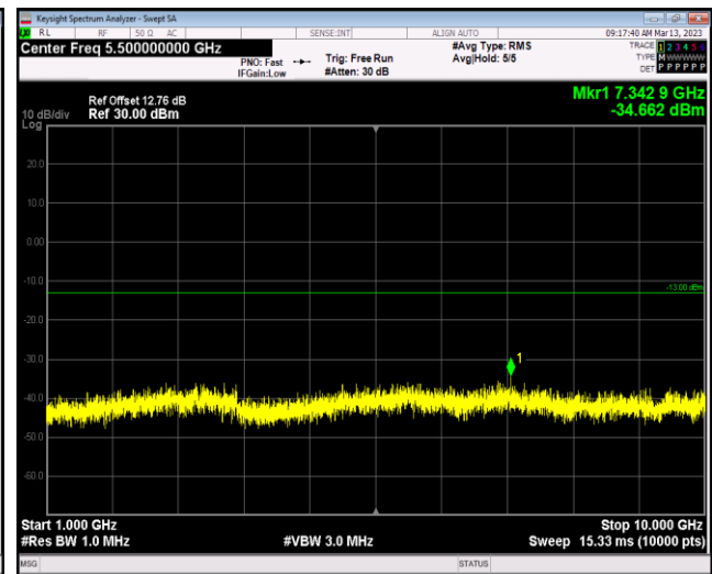
Band5-10MHz-64QAM-20450-1RB#0-Range2:1000~10000MHz
