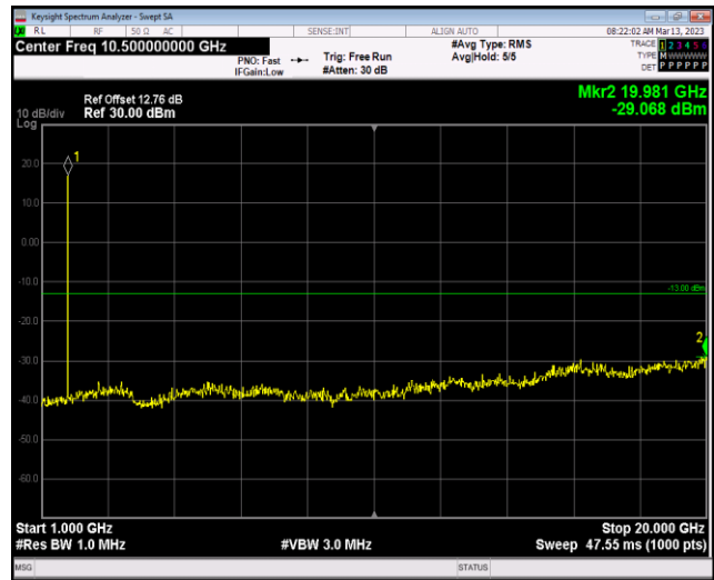
Band4-1.4MHz-64QAM-19957-1RB#0-Range2:1000~20000MHz
