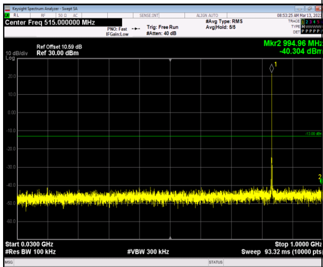
Band5-1.4MHz-16QAM-20643-1RB#0-Range1:30~1000MHz
