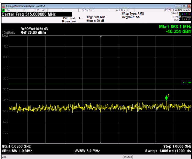
Band7-5MHz-64QAM-21425-1RB#0-Range1:30~1 000MHz
