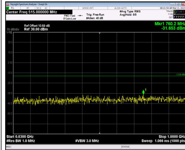
Band4-1.4MHz-64QAM-19957-1RB#0-Range1:30~1000MHz
