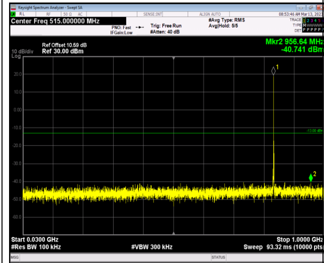
Band5-1.4MHz-64QAM-20643-1RB#0-Range1:30~1000MHz
