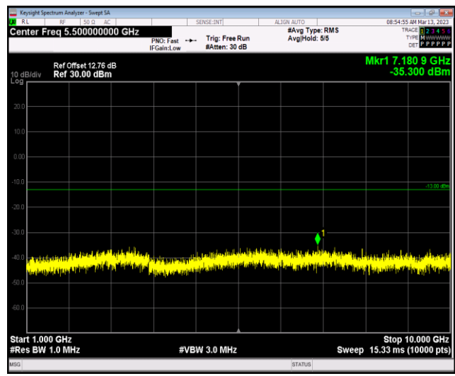
Band5-1.4MHz-64QAM-20643-1RB#0-Range2:1000~10000MHz
