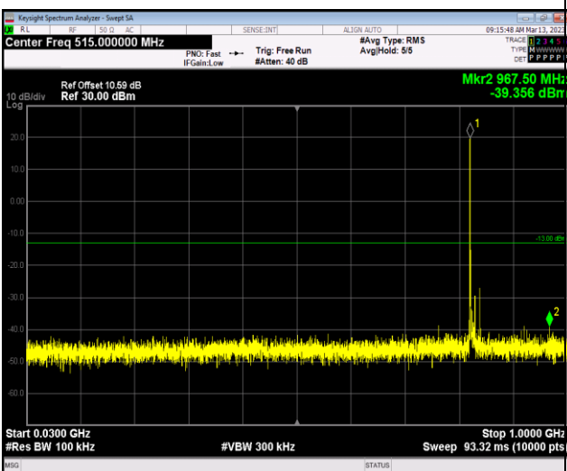
Band5-10MHz-64QAM-20525-1RB#0-Range1:30~1000MHz
