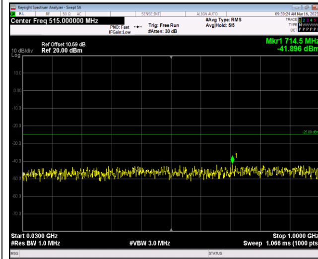
Band7-5MHz-16QAM-21425-1RB#0-Range1:30~1 000MHz
