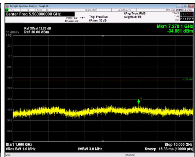
Band5-10MHz-64QAM-20525-1RB#0-Range2:1000~10000MHz
