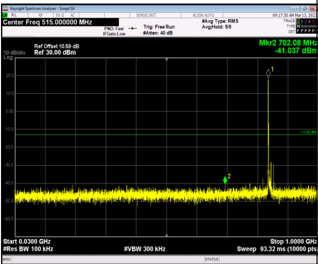
Band5-10MHz-64QAM-20450-1RB#0-Range1:30~1000MHz
