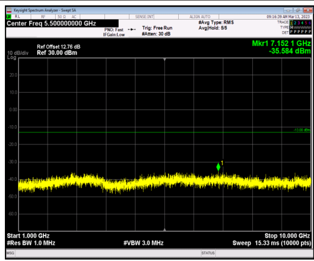
Band5-10MHz-16QAM-20525-1RB#0-Range2:1000~10000MHz
