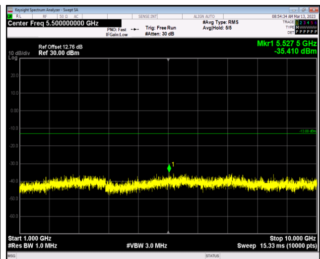
Band5-1.4MHz-64QAM-20407-1RB#0-Range2:1000~10000MHz
