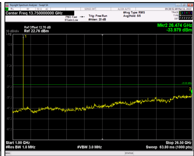
Band7-5MHz-64QAM-21100-1RB#0-Range2:1000~26 500MHz
