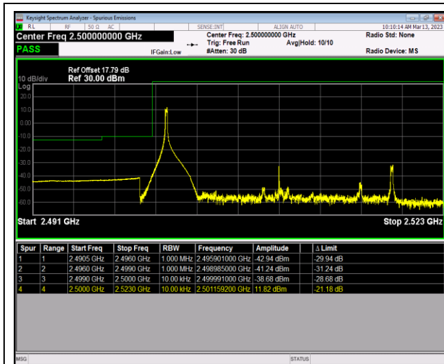
Band7-20MHz-64QAM-20850-100RB#0
