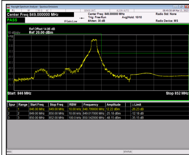
Band5-1.4MHz-64QAM-20407-1RB#0
