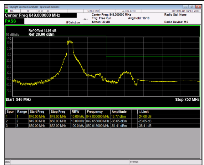
Band5-1.4MHz-QPSK-20643-6RB#0
