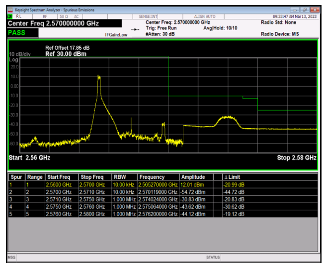
Band7-5MHz-64QAM-21425-25RB#0
