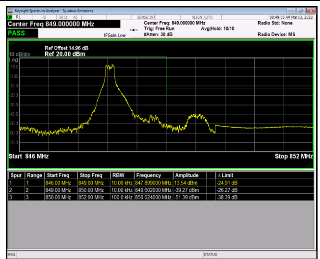
Band5-1.4MHz-16QAM-20643-6RB#0
