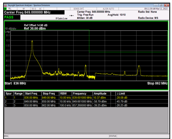
Band5-10MHz-64QAM-20600-50RB#0
