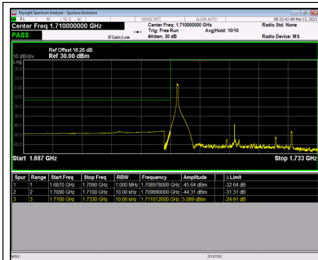
Band4-20MHz-64QAM-20050-100RB#0
