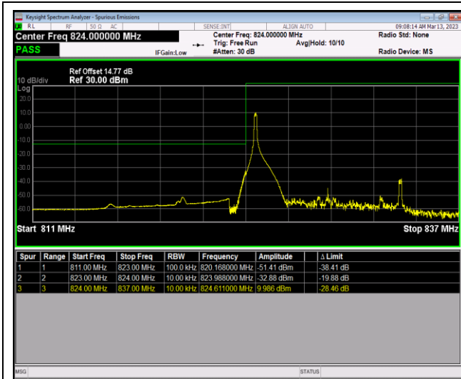
Band5-10MHz-64QAM-20450-50RB#0
