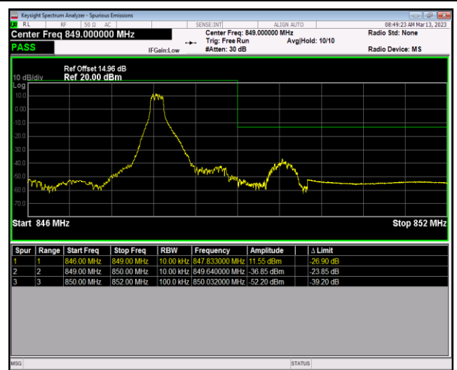
Band5-1.4MHz-64QAM-20643-6RB#0
