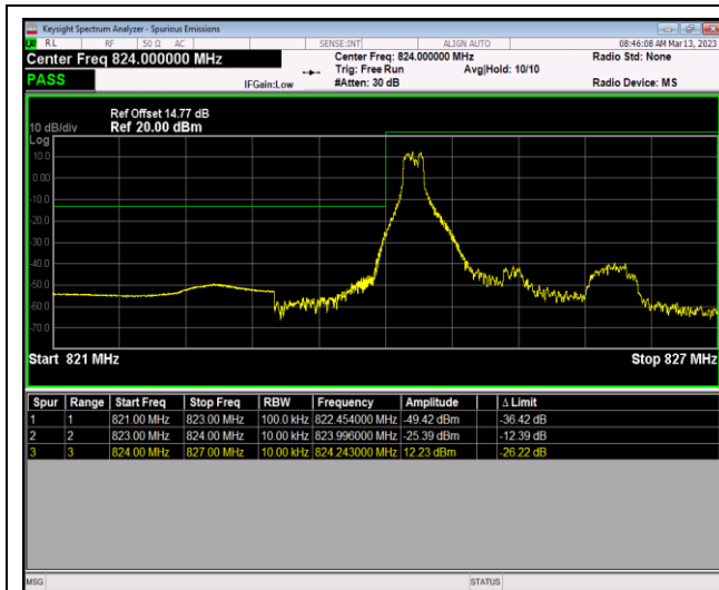
Band5-1.4MHz-64QAM-20407-6RB#0
