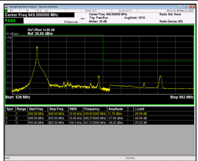
Band5-10MHz-16QAM-20600-50RB#0
