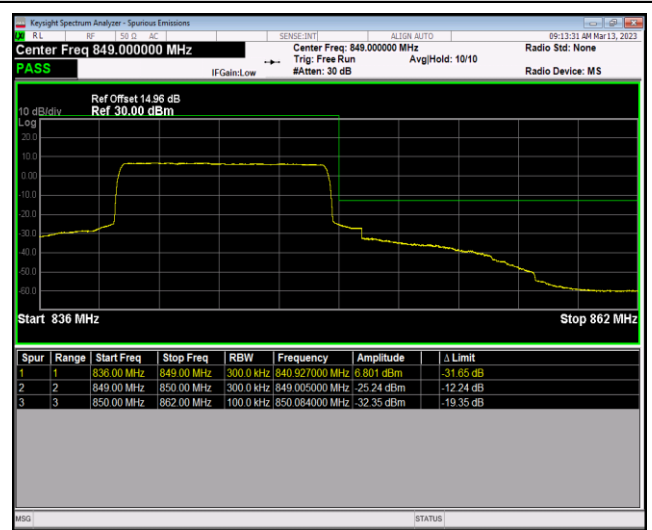
Band5-10MHz-16QAM-20450-1RB#49
