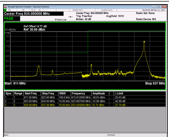
Band5-10MHz-16QAM-20600-1RB#0
