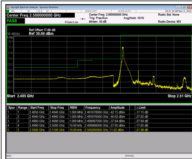
Band7-5MHz-64QAM-20775-25RB#0
