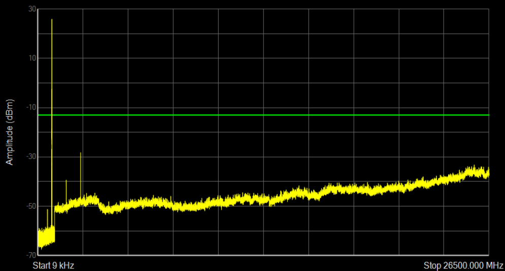
Band26(824-849) 16QAM BW=5MHz Channel=27015 RB Size=1 Position=#0
