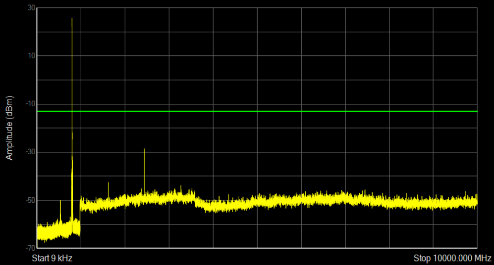
Band26(814-824) QPSK BW=3MHz Channel=26775 RB Size=1 Position=#0
