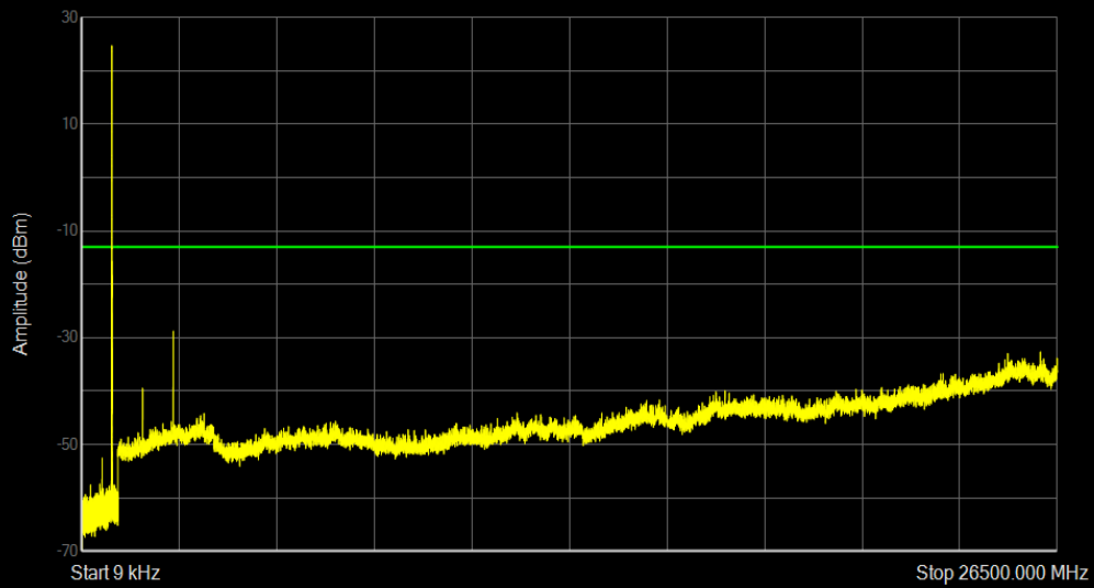
Band26(824-849) 16QAM BW=5MHz Channel=26915 RB Size=1 Position=#0
