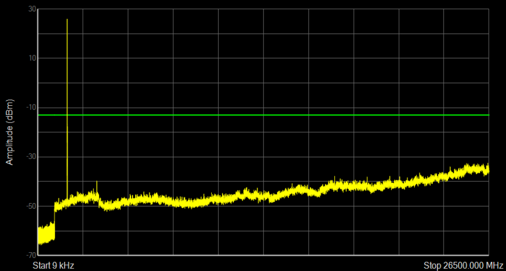
Band66 QAM16 BW=10MHz Channel=132322 RB Size=1 Position=#0
