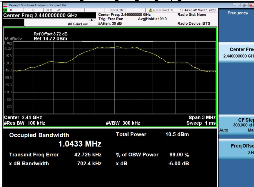
-6dB_Bandwidth_NVNT_ANT1_1Mbps_2440
