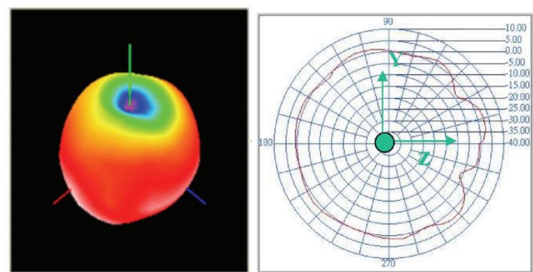
2.4GHz Gain:2.41dBi Efficiency:75.6 1%
