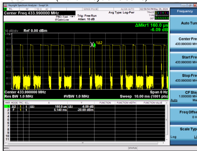
(Time per burst: 0.16ms*14pcs)
