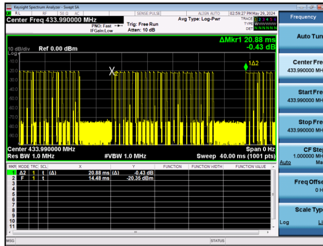
(Transmit cycle 20.88ms)
