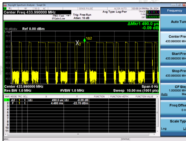
(Time per burst: 0.49ms*11pcs)
