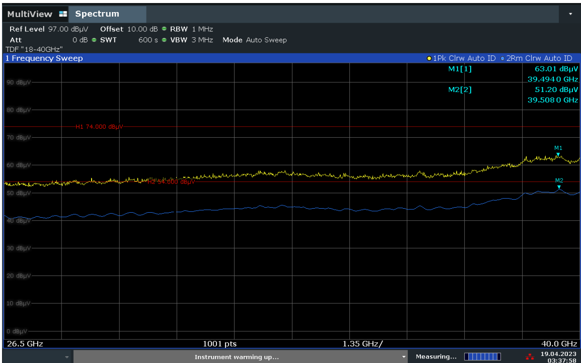
Plots No. 4: 26 GHz to 40 GHz, Horizontal / Vertical Polarization
