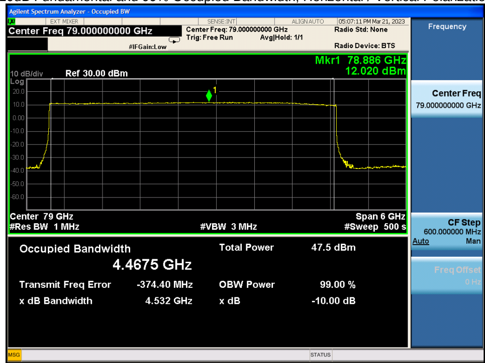
Plots No. 11: 10dB Fundamental and 99% Occupied Bandwidth, Horizontal / Vertical Polarization_ V nor /T nor
