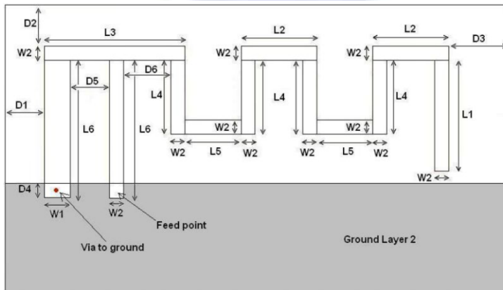
Figure 3: Antenna Dimensions
