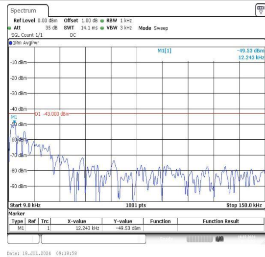
Band66_15MHz_16QAM_132322_1RB#0_0.009~ 0.15_0.009~0.15
