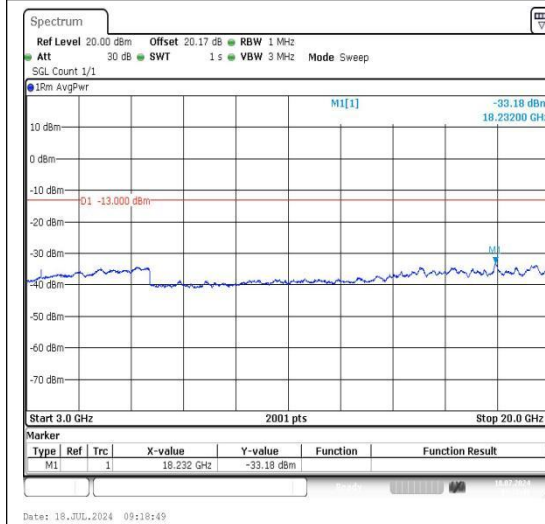
Band66_15MHz_QPSK_132322_1RB#0_3000~2 0000_3000~20000
