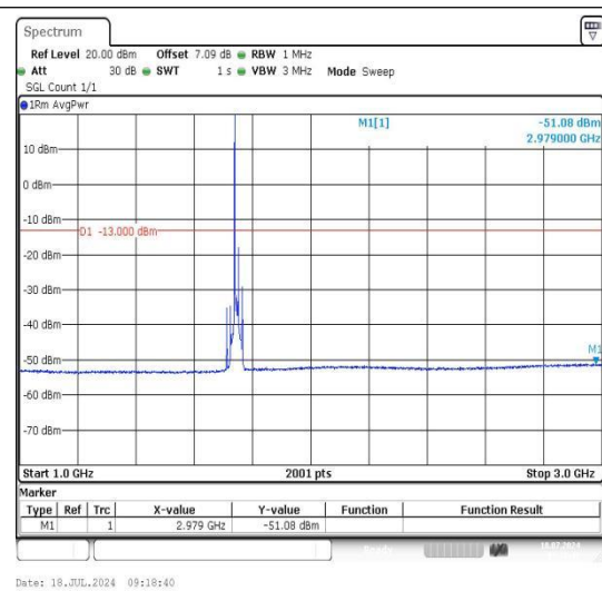
Band66_15MHz_QPSK_132322_1RB#0_1000~30 00_1000~3000
