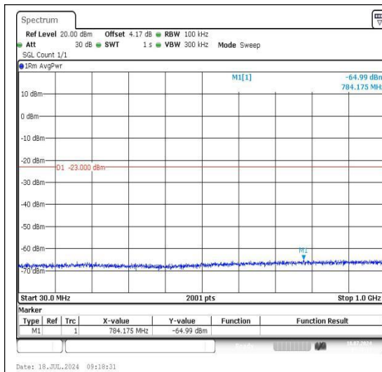
Band66_15MHz_QPSK_132322_1RB#0_30~100 0_30~1000
