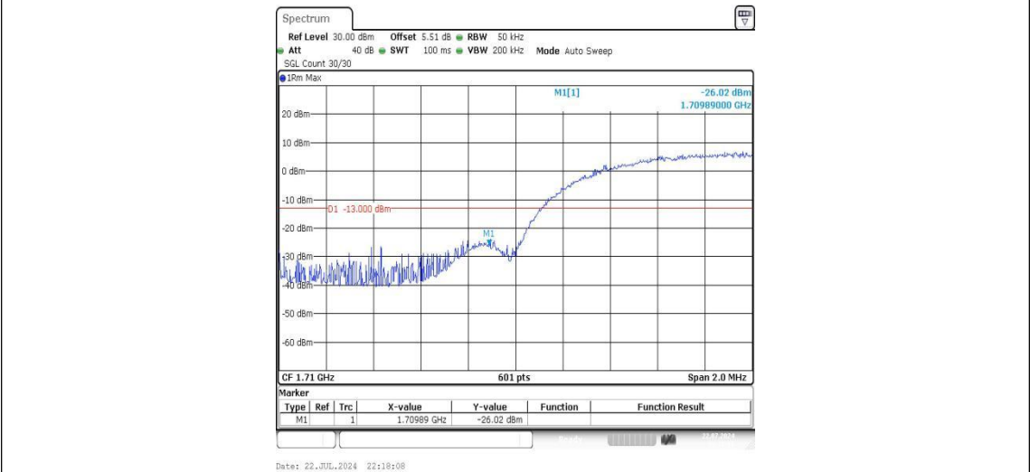
Band4-1312-PASS
