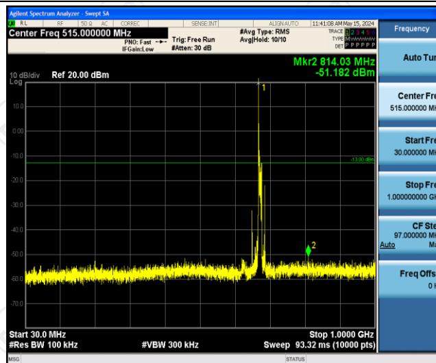
Band71-10MHz-16QAM-133297-1RB#0-Range1:30~1000MHz
