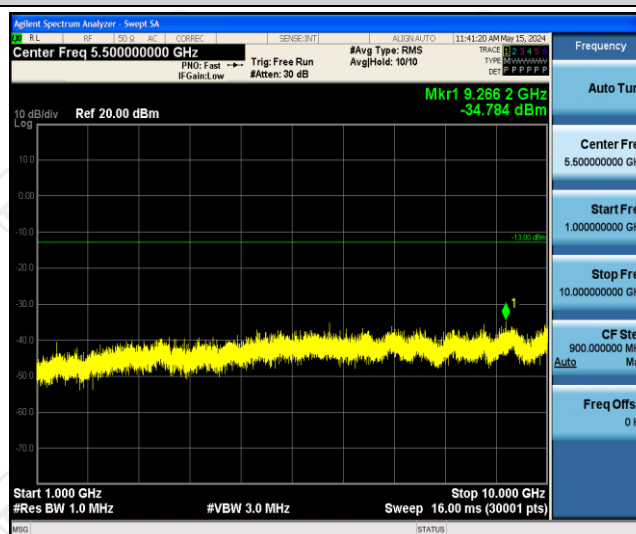
Band71-10MHz-16QAM-133297-1RB#0-Range2:1000~10000MHz
