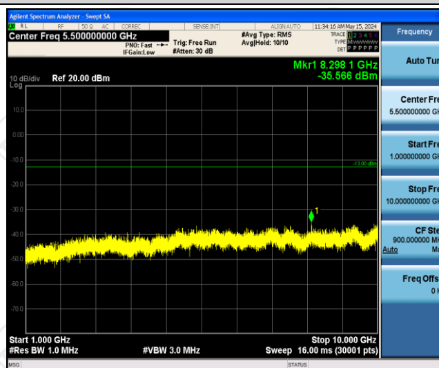
Band71-5MHz-16QAM-133297-1RB#0-Range2:1000~10000MHz
