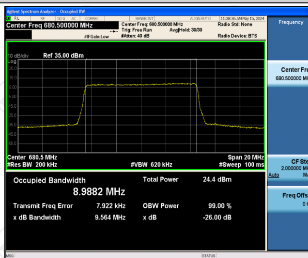
Band71-10MHz-QPSK-133297-50RB#0
