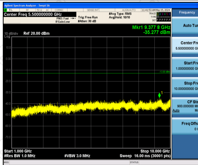
Band71-10MHz-QPSK-133422-1RB#0-Range2:1000~10000MHz
