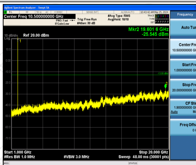
Band66-3MHz-16QAM-132657-1RB#0-Range2:1000~20000MHz
