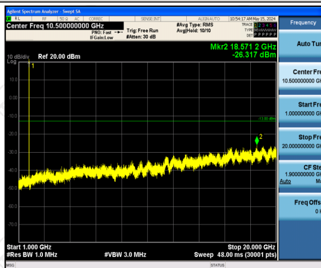
Band66-5MHz-QPSK-132647-1RB#0-Range2:1000~20000MHz
