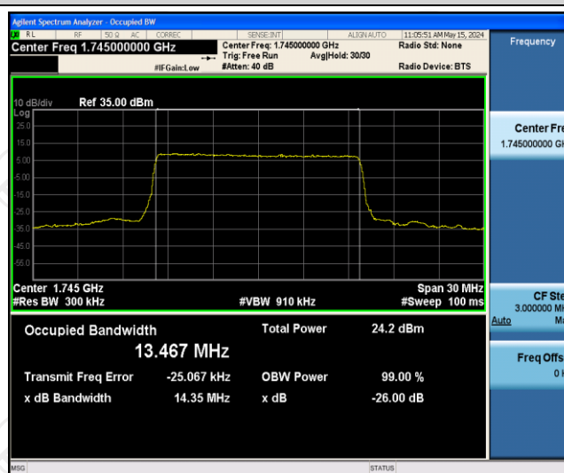
Band66-15MHz-QPSK-132322-75RB#0
