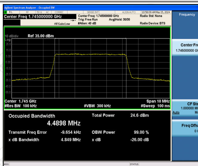
Band66-5MHz-QPSK-132322-25RB#0
