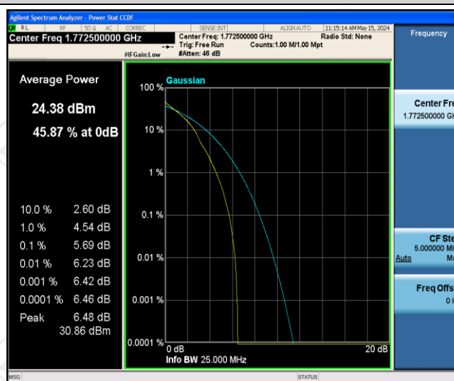
Band66-15MHz-QPSK-132597-1RB#0
