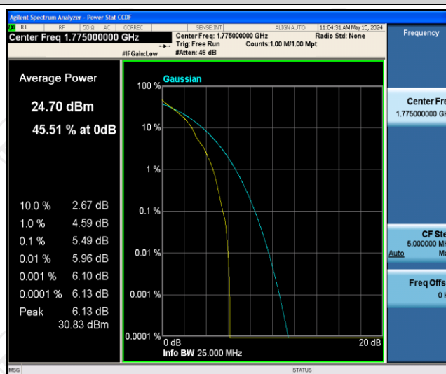
Band66-10MHz-QPSK-132622-1RB#0
