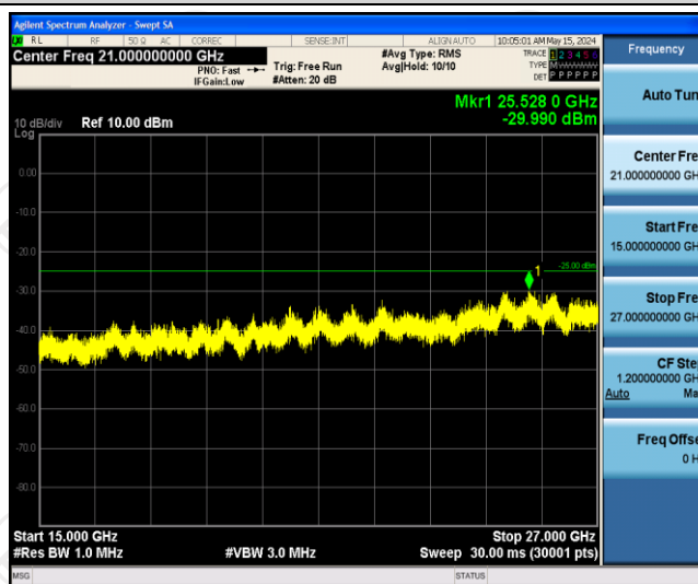
Band41-15MHz-QPSK-39725-1RB#0-Range3:15000~27000MHz
