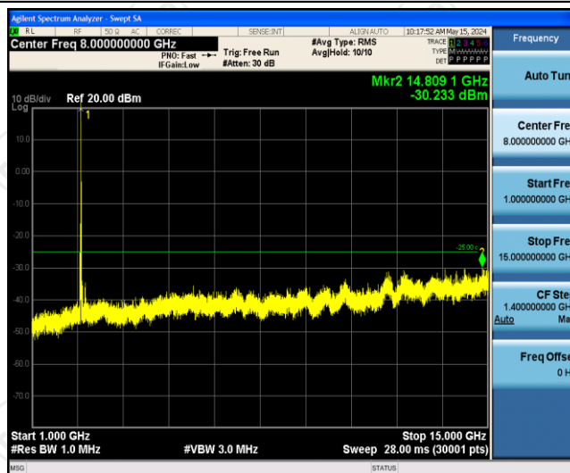
Band41-20MHz-16QAM-39750-1RB#0-Range2:1000~15000MHz
