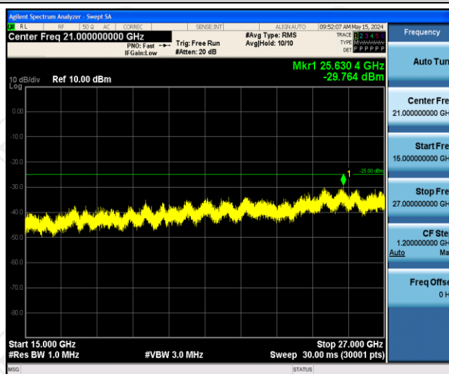
Band41-5MHz-16QAM-41565-1RB#0-Range3:15000~27000MHz
