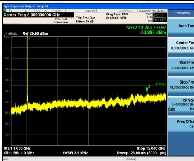
Band41-20MHz-QPSK-39750-1RB#0-Range2:1000~15000MHz
