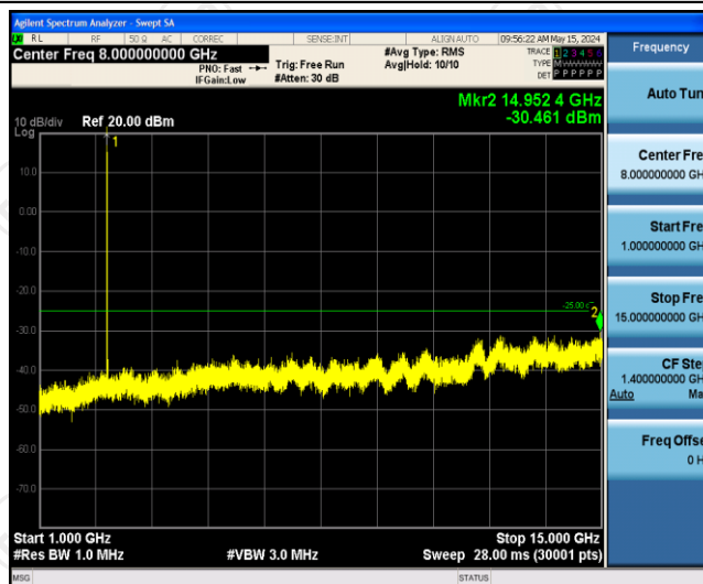
Band41-10MHz-16QAM-41540-1RB#0-Range2:1000~15000MHz
