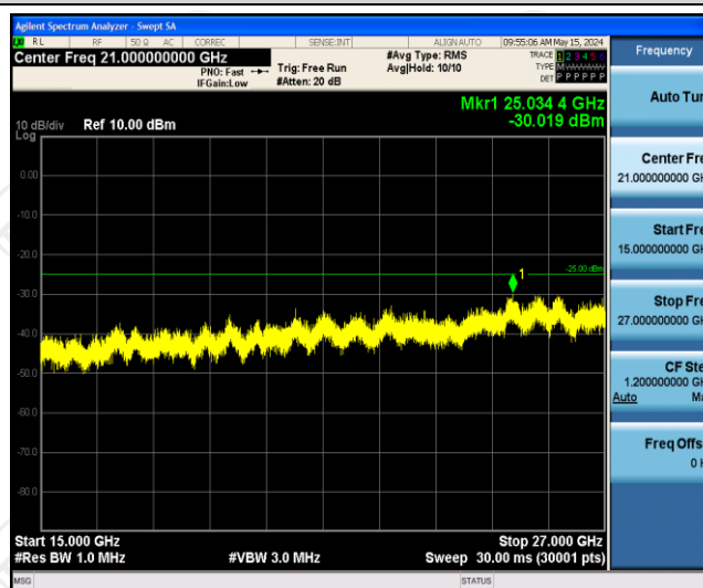
Band41-10MHz-16QAM-40620-1RB#0-Range3:15000~27000MHz
