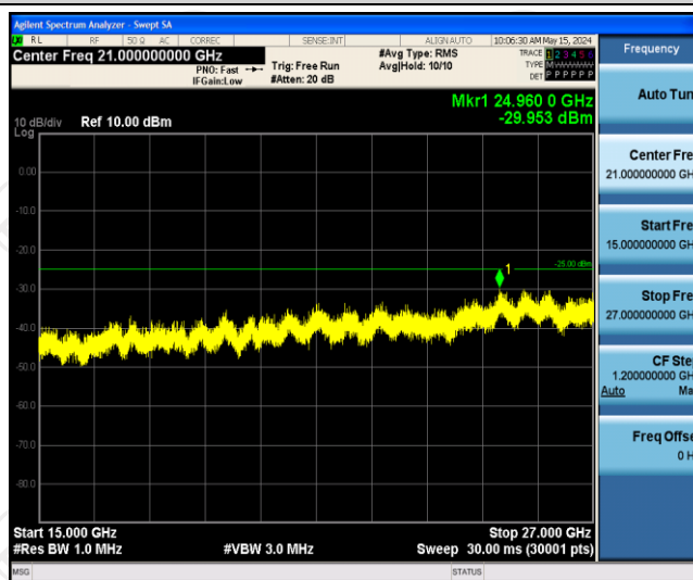
Band41-15MHz-QPSK-40620-1RB#0-Range3:15000~27000MHz
