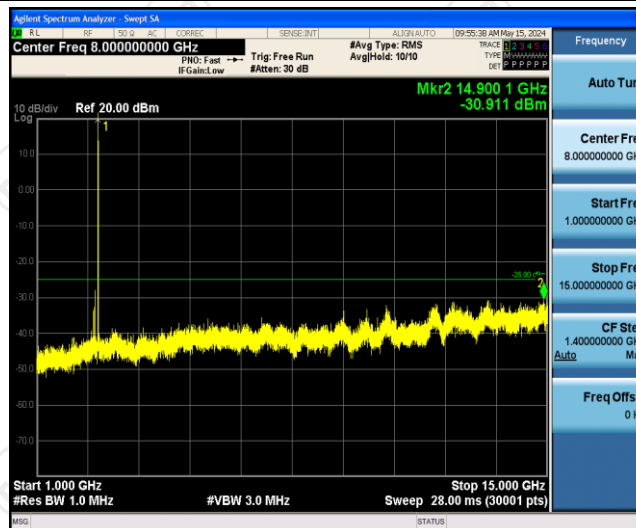
Band41-10MHz-QPSK-41540-1RB#0-Range2:1000~15000MHz
