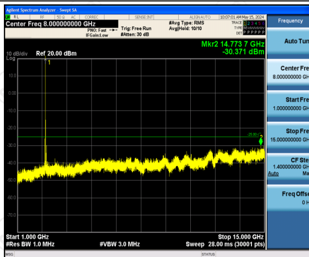
Band41-15MHz-16QAM-40620-1RB#0-Range2:1000~15000MHz
