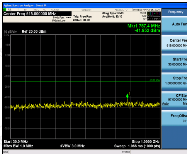
Band41-5MHz-16QAM-41565-1RB#0-Range1:30~1000MHz
