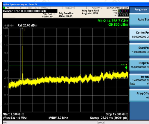
Band41-20MHz-16QAM-40620-1RB#0-Range2:1000~15000MHz
