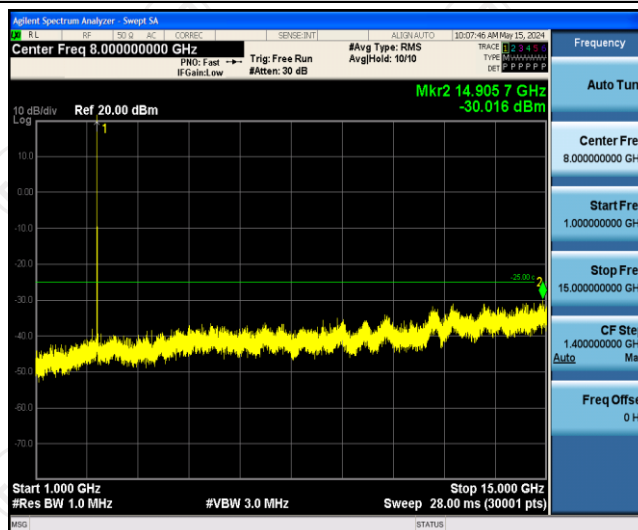
Band41-15MHz-QPSK-41515-1RB#0-Range2:1000~15000MHz
