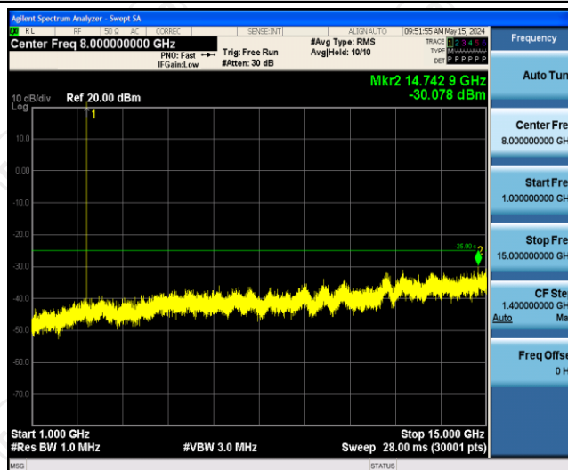
Band41-5MHz-16QAM-41565-1RB#0-Range2:1000~15000MHz
