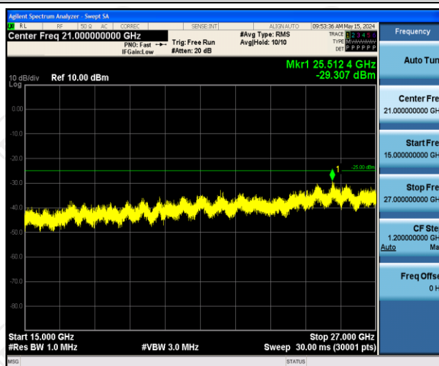
Band41-10MHz-16QAM-39700-1RB#0-Range3:15000~27000MHz
