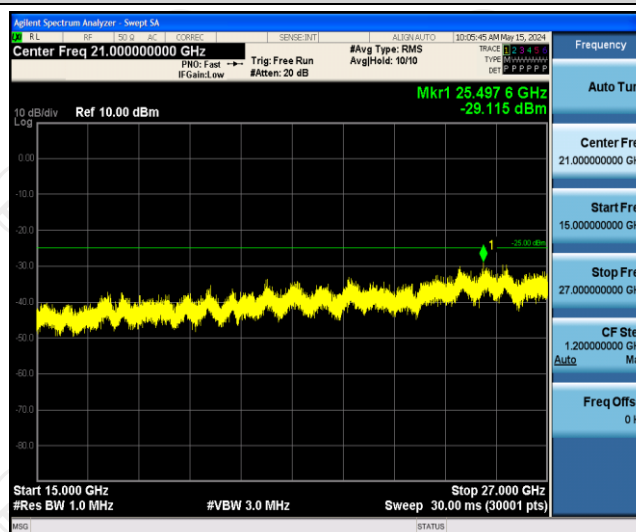
Band41-15MHz-16QAM-39725-1RB#0-Range3:15000~27000MHz
