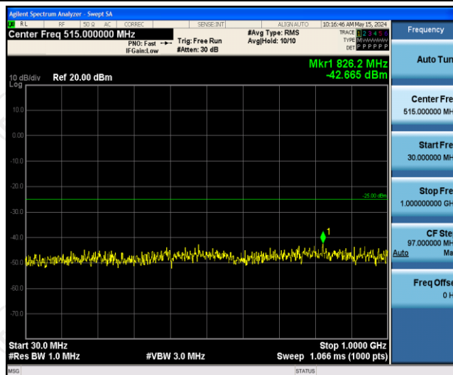
Band41-20MHz-QPSK-39750-1RB#0-Range1:30~1000MHz
