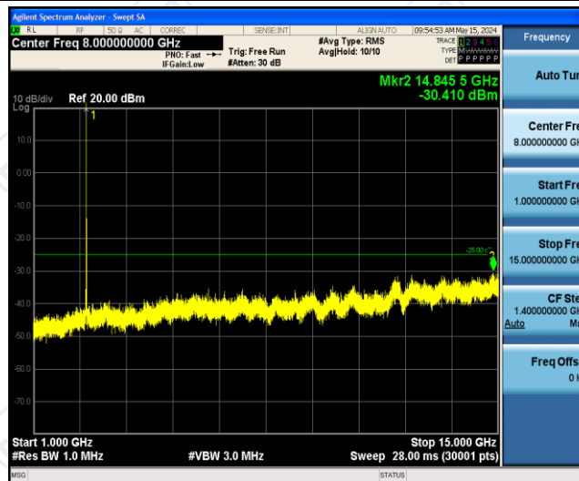
Band41-10MHz-16QAM-40620-1RB#0-Range2:1000~15000MHz
