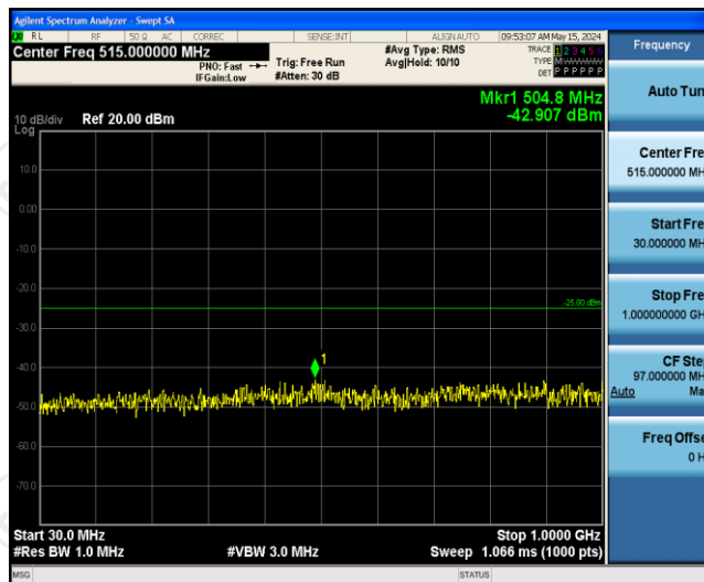
Band41-10MHz-16QAM-39700-1RB#0-Range1:30~1000MHz
