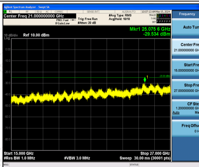
Band41-15MHz-16QAM-40620-1RB#0-Range3:15000~27000MHz
