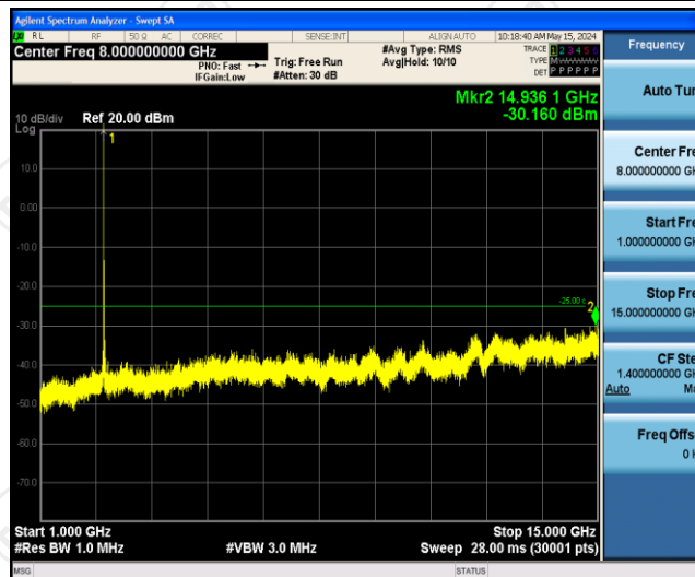
Band41-20MHz-QPSK-40620-1RB#0-Range2:1000~15000MHz
