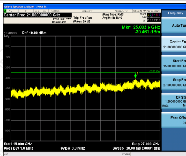
Band41-20MHz-16QAM-40620-1RB#0-Range3:15000~27000MHz
