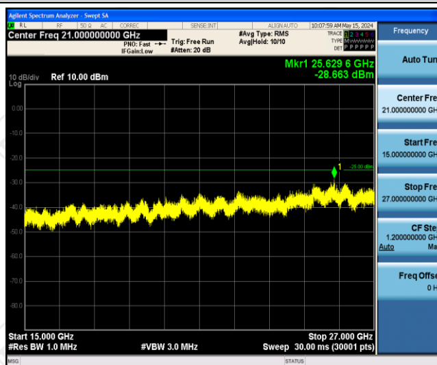
Band41-15MHz-QPSK-41515-1RB#0-Range3:15000~27000MHz
