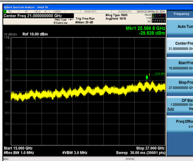
Band41-10MHz-QPSK-40620-1RB#0-Range3:15000~27000MHz
