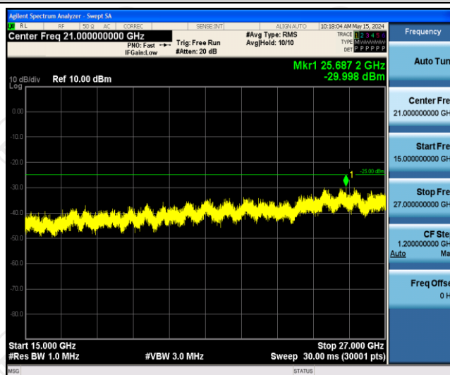
Band41-20MHz-16QAM-39750-1RB#0-Range3:15000~27000MHz
