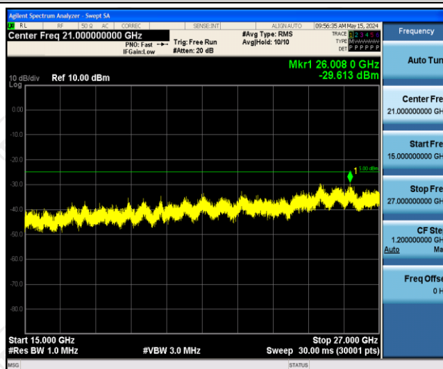
Band41-10MHz-16QAM-41540-1RB#0-Range3:15000~27000MHz
