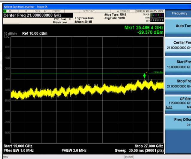
Band41-15MHz-16QAM-41515-1RB#0-Range3:15000~27000MHz
