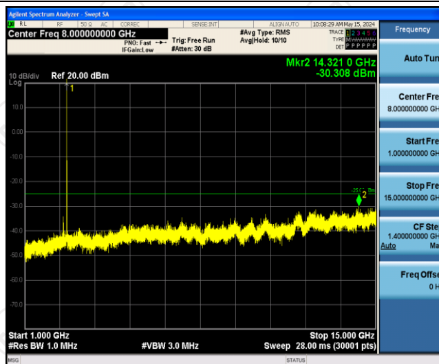
Band41-15MHz-16QAM-41515-1RB#0-Range2:1000~15000MHz
