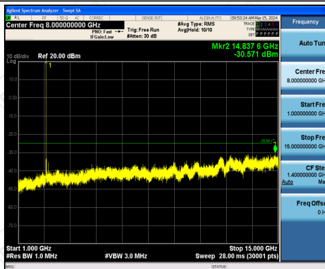
Band41-10MHz-16QAM-39700-1RB#0-Range2:1000~15000MHz
