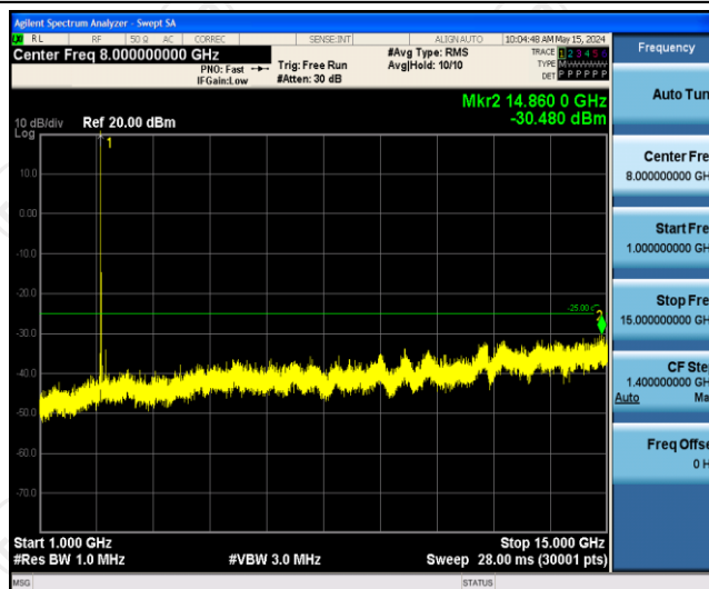
Band41-15MHz-QPSK-39725-1RB#0-Range2:1000~15000MHz
