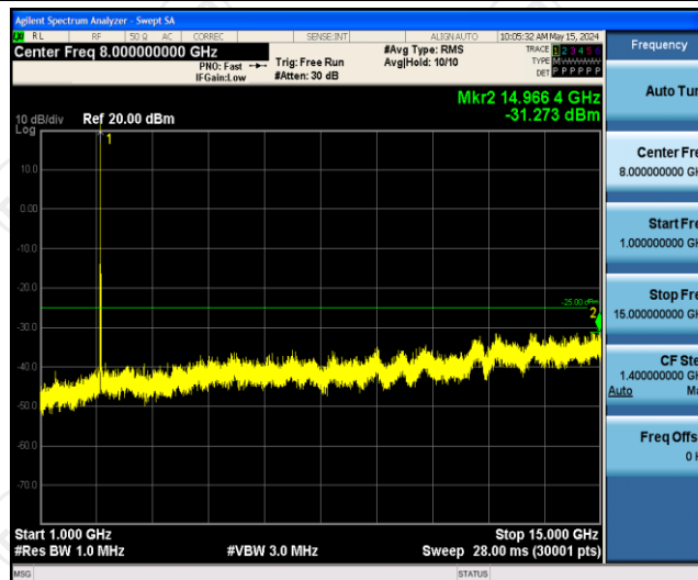
Band41-15MHz-16QAM-39725-1RB#0-Range2:1000~15000MHz
