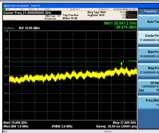
Band41-20MHz-QPSK-40620-1RB#0-Range3:15000~27000MHz
