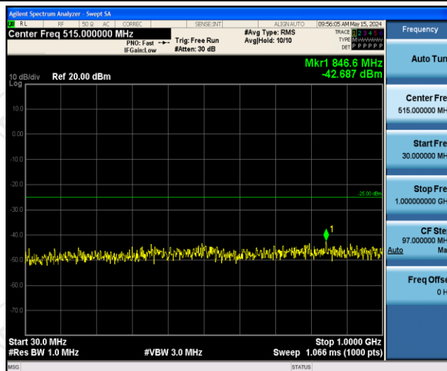
Band41-10MHz-16QAM-41540-1RB#0-Range1:30~1000MHz
