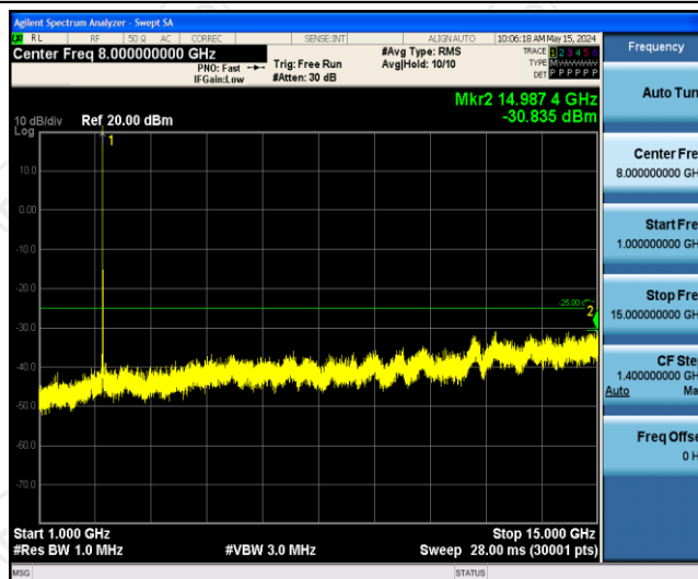
Band41-15MHz-QPSK-40620-1RB#0-Range2:1000~15000MHz
