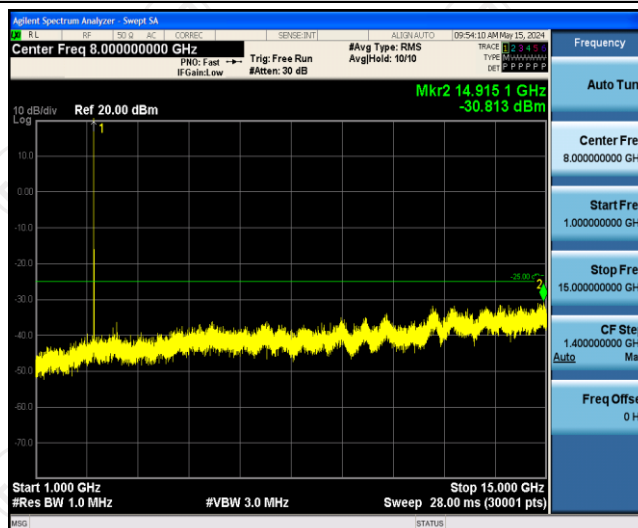
Band41-10MHz-QPSK-40620-1RB#0-Range2:1000~15000MHz
