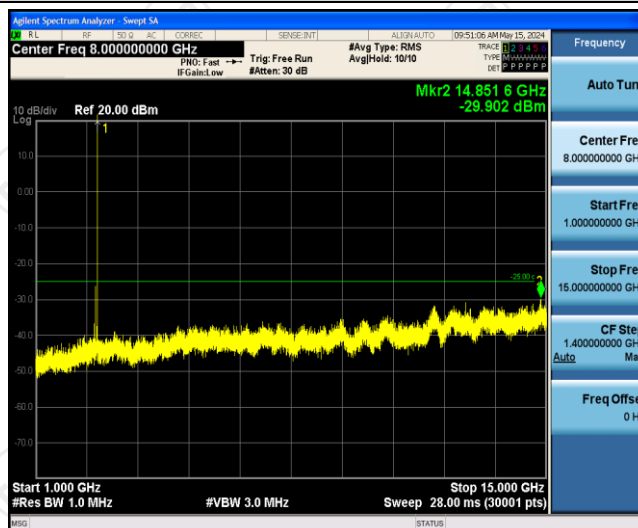
Band41-5MHz-QPSK-41565-1RB#0-Range2:1000~15000MHz
