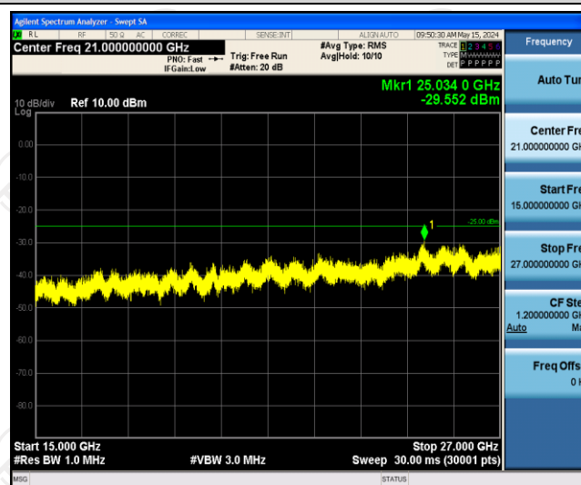
Band41-5MHz-16QAM-40620-1RB#0-Range3:15000~27000MHz
