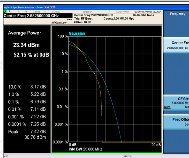
Band41-15MHz-QPSK-41515-1RB#0
