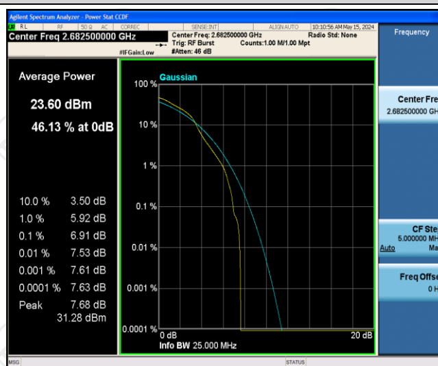
Band41-15MHz-16QAM-41515-1RB#0
