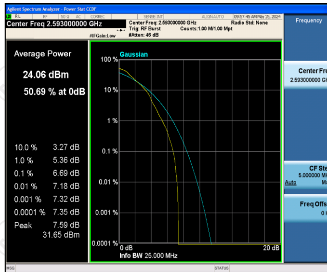
Band41-10MHz-QPSK-40620-1RB#0
