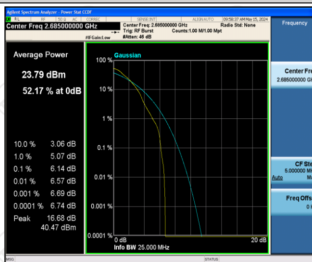
Band41-10MHz-QPSK-41540-1RB#0
