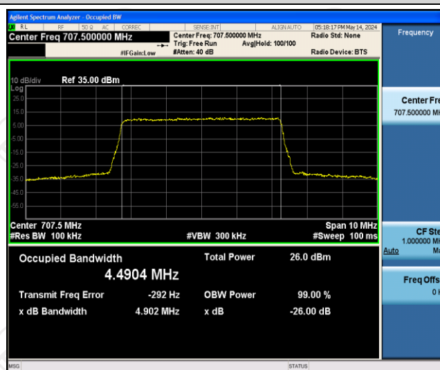
Band12-5MHz-QPSK-23095-25RB#0
