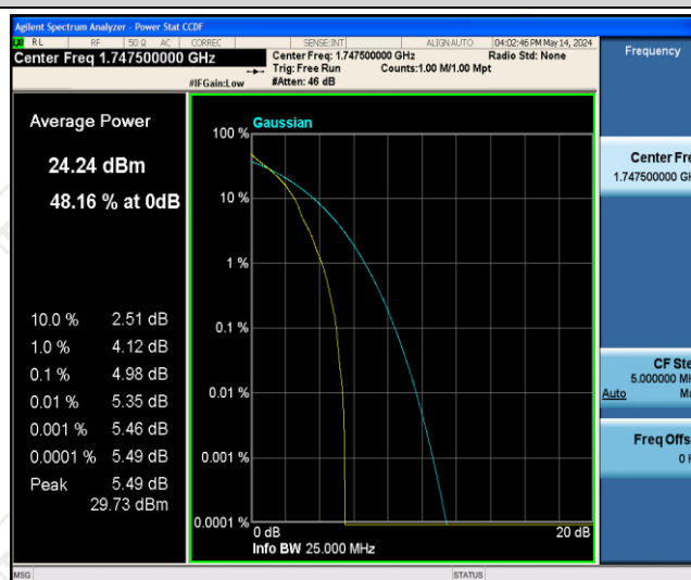
Band4-15MHz-QPSK-20325-1RB#0
