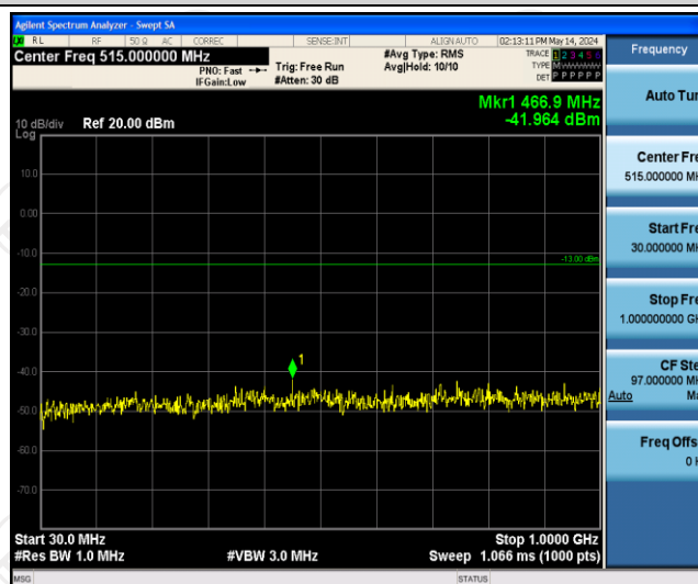
Band2-1.4MHz-16QAM-18900-1RB#0-Range1:30~1000MHz
