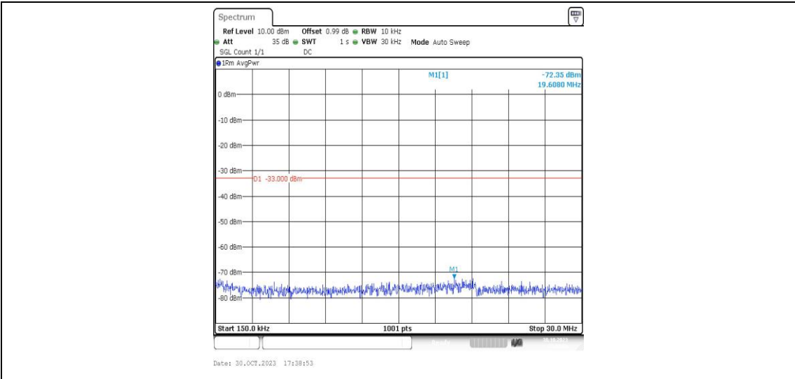
Band2-9538-5-0.15~30MHz-PASS
