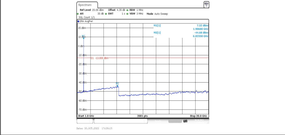
Band2-9538-5-1000~20000MHz-PASS
