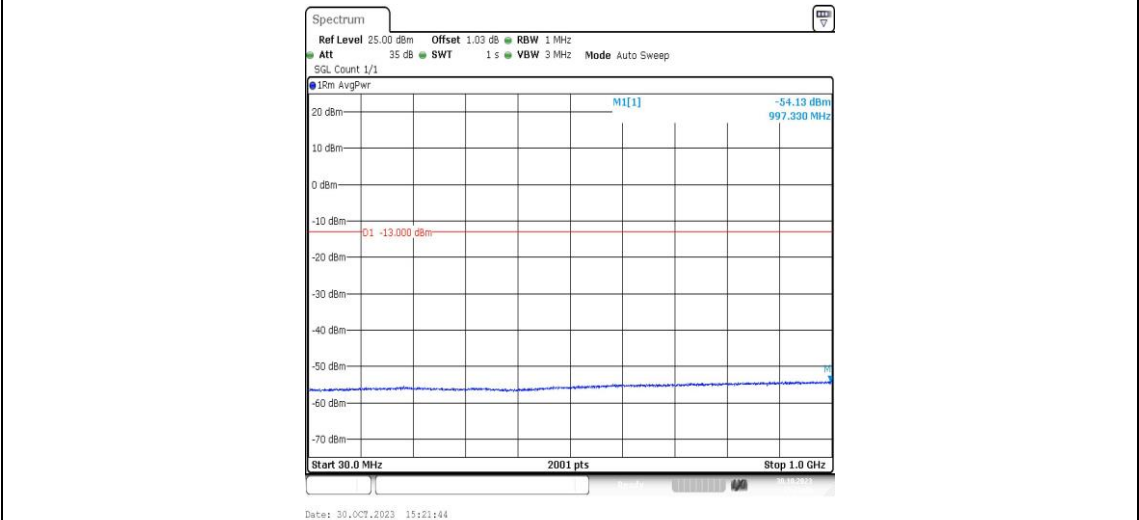
Band2-9262-4-30~1000MHz-PASS
