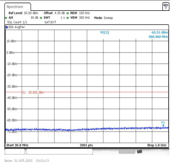
Band41_20MHz_16QAM_41490_1RB#0_30~1000_30~1000
