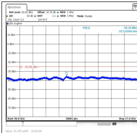
Band41_20MHz_QPSK_41490_1RB#0_20000~27000_20000~27000
