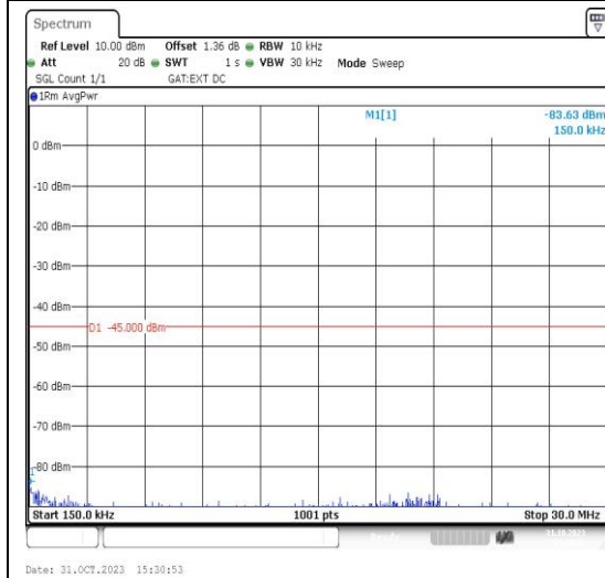
Band41_20MHz_16QAM_41490_1RB#0_0.15~3_0.15~30
