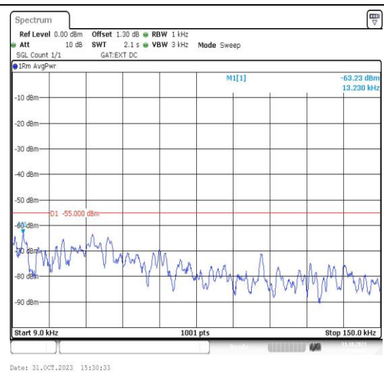
Band41_20MHz_16QAM_41490_1RB#0_0.009~0.15_0.009~0.15
