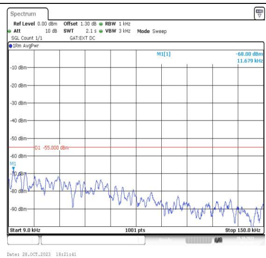
Band41_5MHz_16QAM_40620_1RB#0_0.009~0.15 5_0.009~0.15
