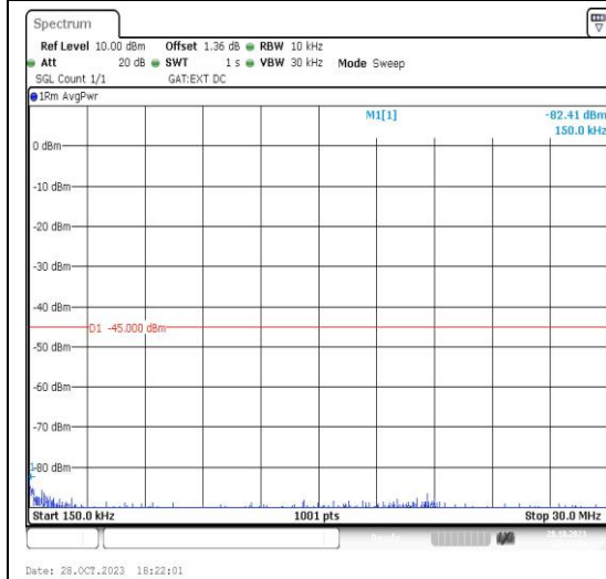
Band41_5MHz_16QAM_40620_1RB#0_0.15~30 _0.15~30
