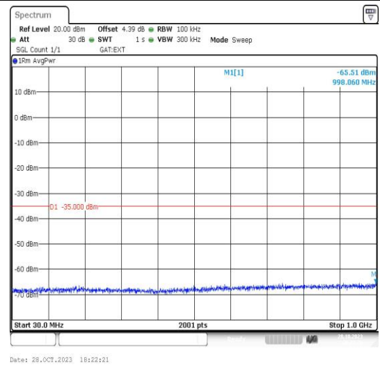
Band41_5MHz_16QAM_40620_1RB#0_30~1000_ 30~1000
