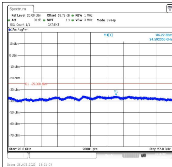
Band41_5MHz_QPSK_40620_1RB#0_20000~27000 000_20000~27000
