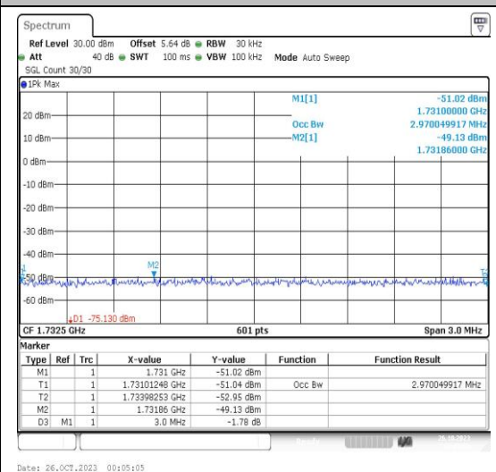
Band4-1.4MHz-16QAM-20175-6RB#0-PASS
