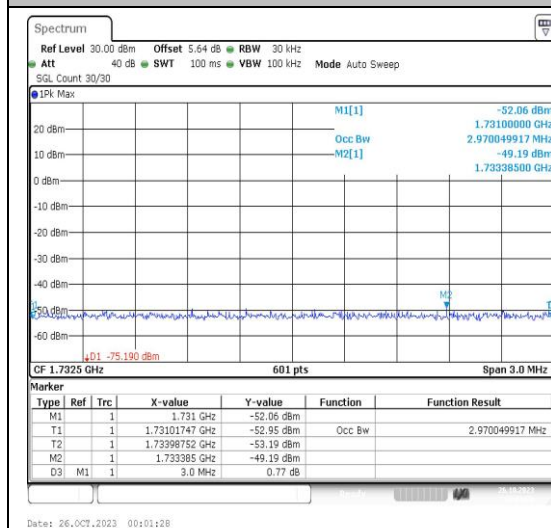
Band4-1.4MHz-QPSK-20175-6RB#0-PASS
