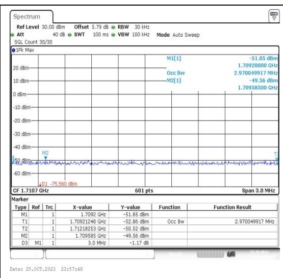
Band4-1.4MHz-16QAM-19957-6RB#0-PASS
