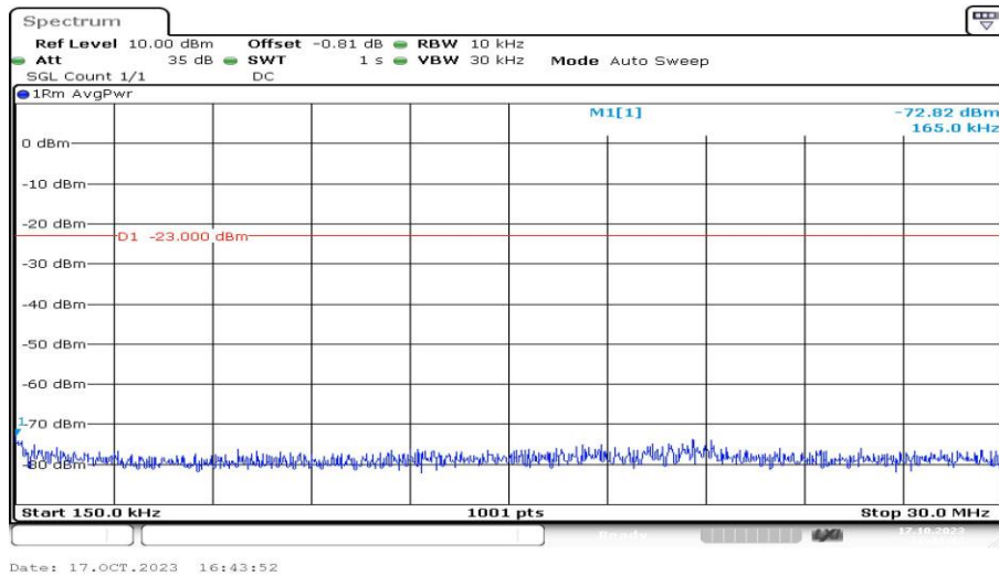
Band5-4233-1-0.15~30MHz-PASS
