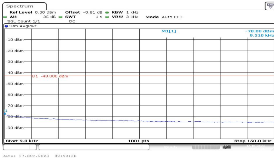
Band2-9400-1-0.009~0.15MHz-PASS
