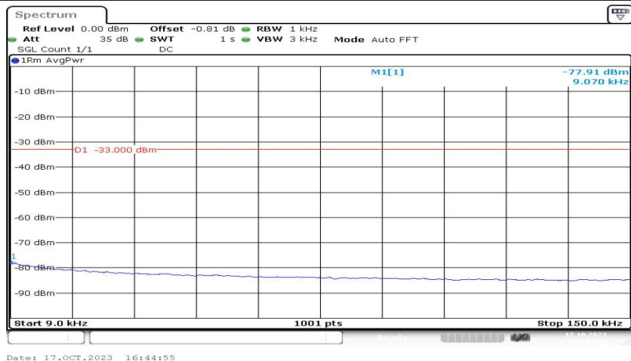
Band5-4132-2-0.009~0.15MHz-PASS
