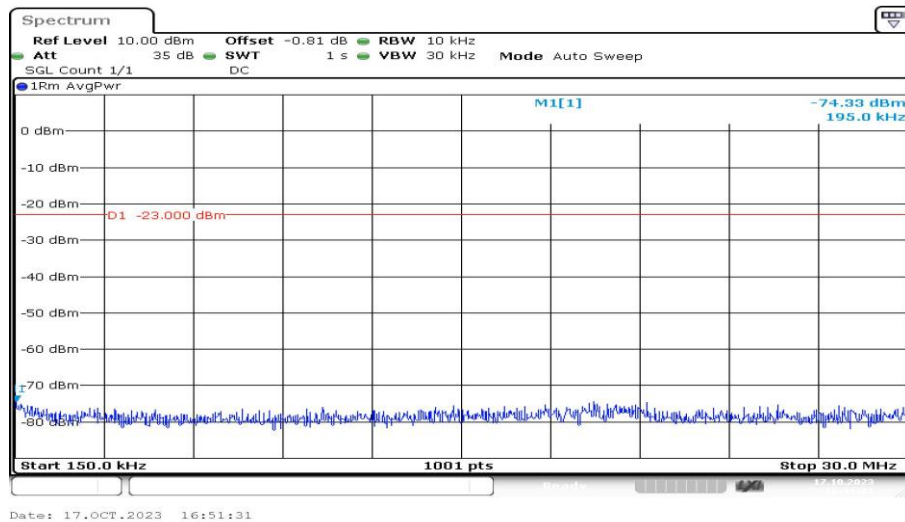
Band5-4132-4-0.15~30MHz-PASS
