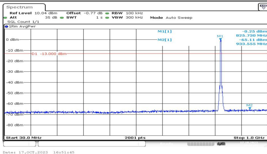
Band5-4132-4-30~1000MHz-PASS
