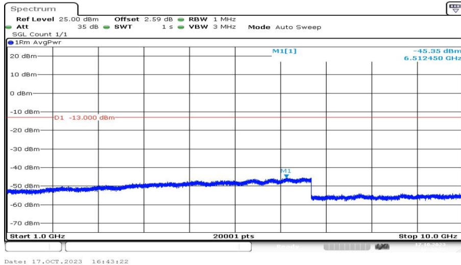
Band5-4182-1-1000~10000MHz-PASS
