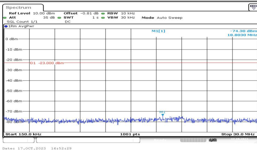
Band5-4182-4-0.15~30MHz-PASS
