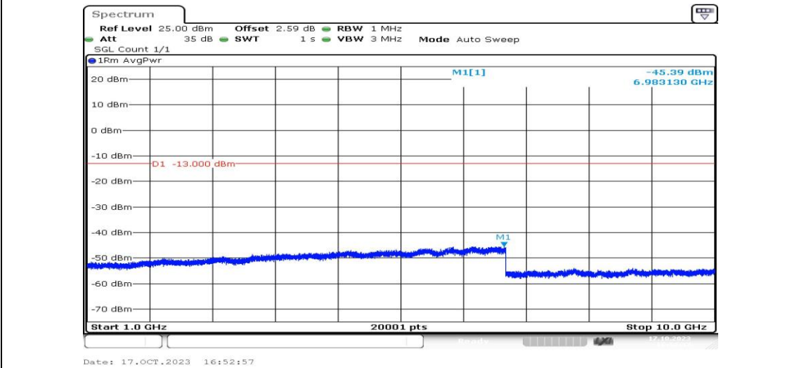
Band5-4182-4-1000~10000MHz-PASS
