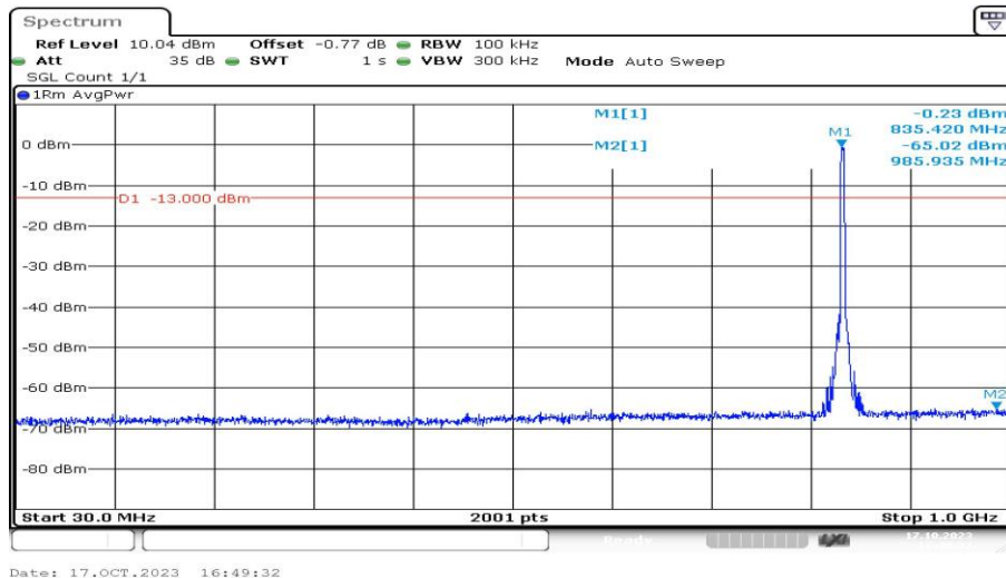
Band5-4182-3-30~1000MHz-PASS
