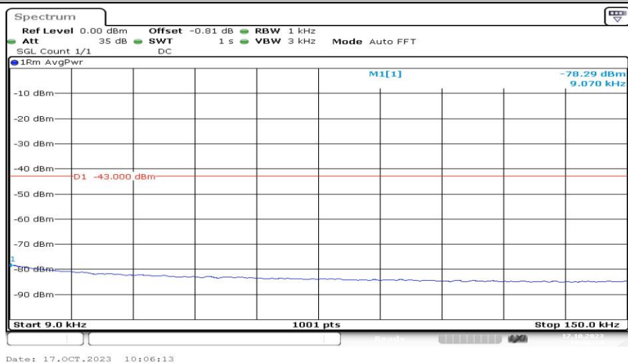
Band2-9538-2-0.009~0.15MHz-PASS
