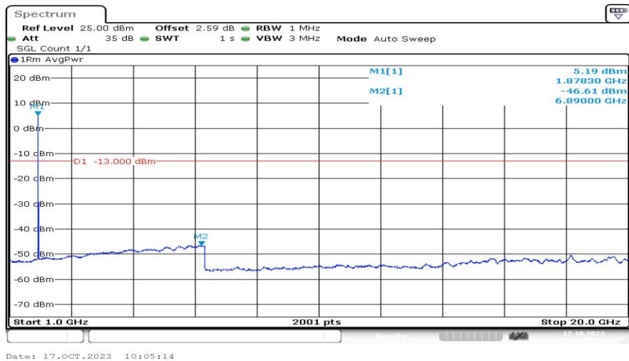
Band2-9400-2-1000~20000MHz-PASS
