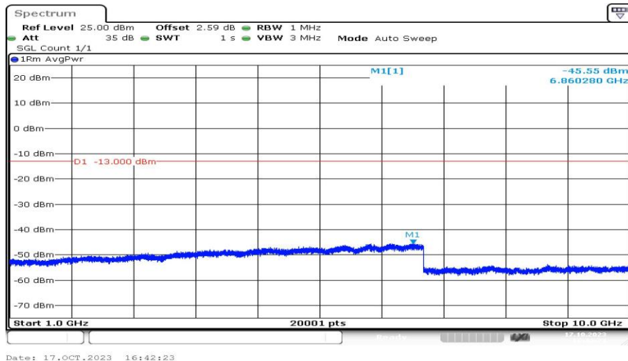
Band5-4132-1-1000~10000MHz-PASS
