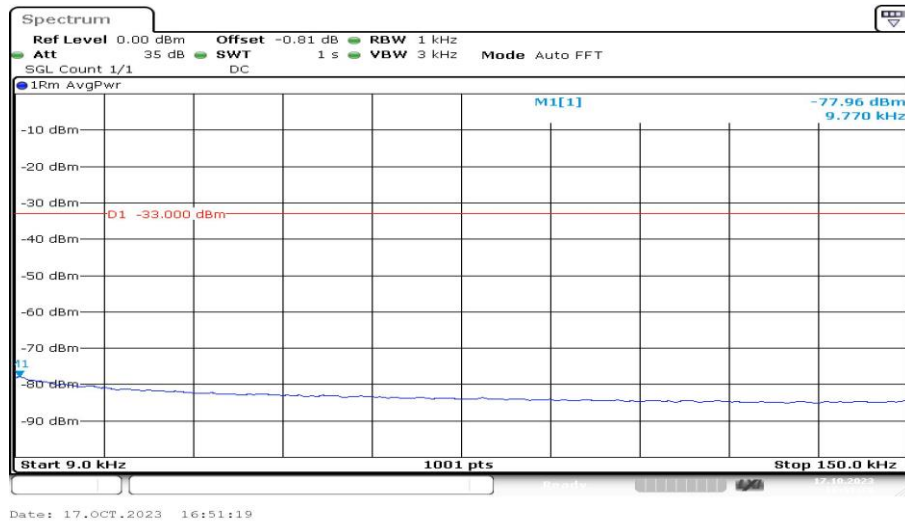
Band5-4132-4-0.009~0.15MHz-PASS
