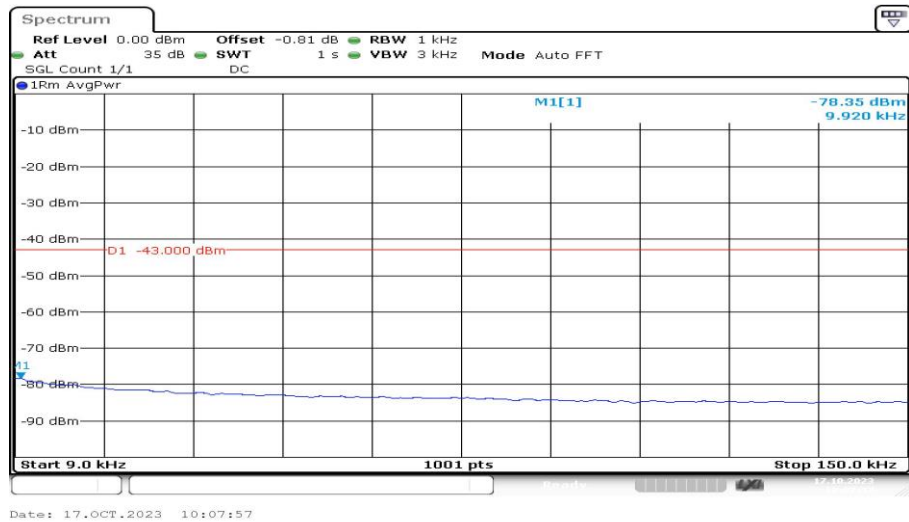
Band2-9262-3-0.009~0.15MHz-PASS
