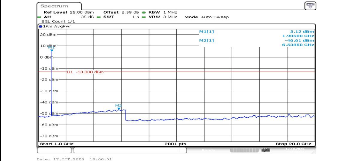
Band2-9538-2-1000~20000MHz-PASS
