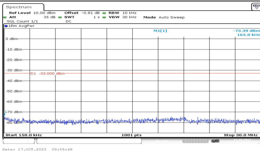
Band2-9400-1-0.15~30MHz-PASS
