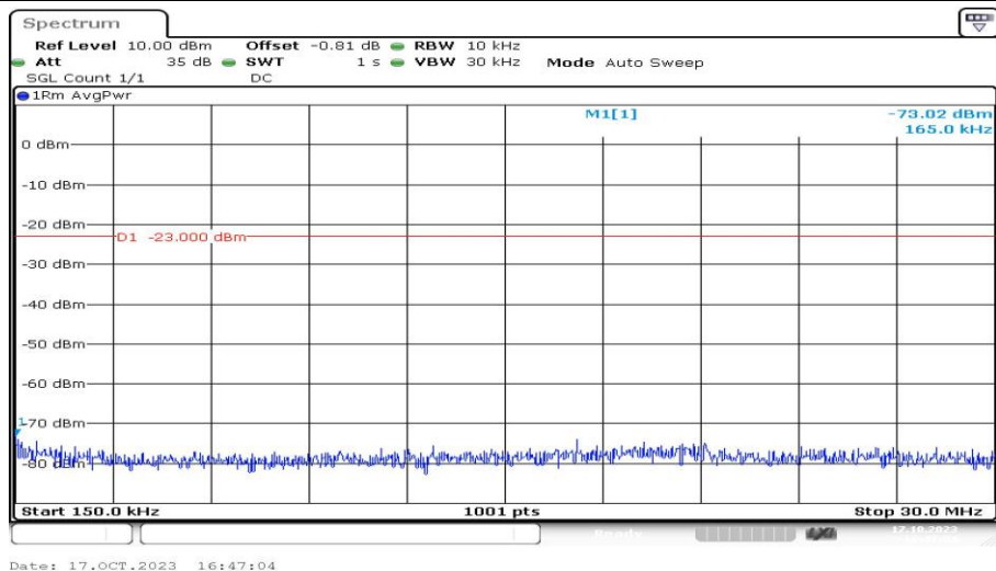
Band5-4233-2-0.15~30MHz-PASS
