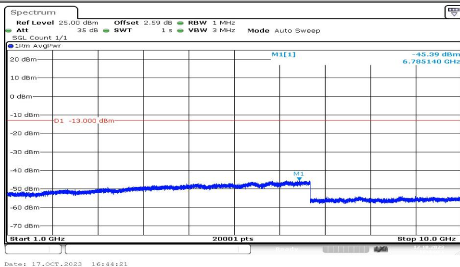
Band5-4233-1-1000~10000MHz-PASS
