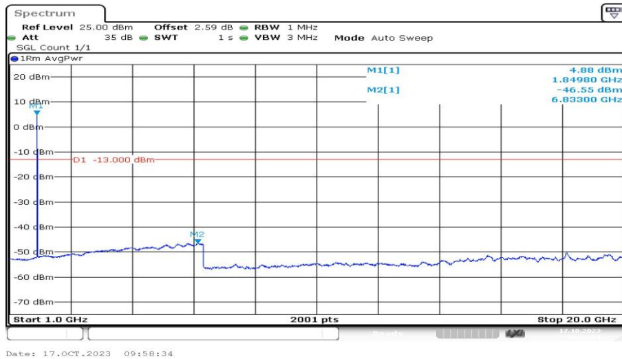
Band2-9262-1-1000~20000MHz-PASS
