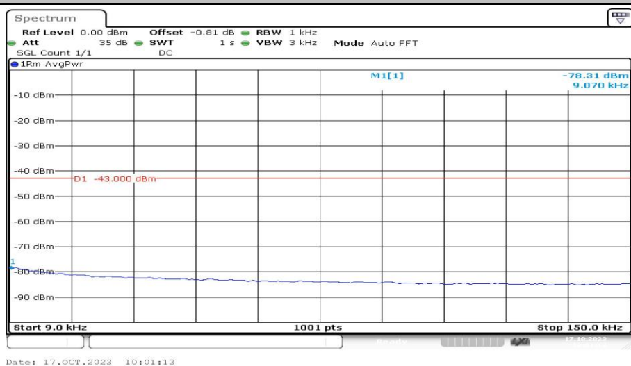
Band2-9538-1-0.009~0.15MHz-PASS
