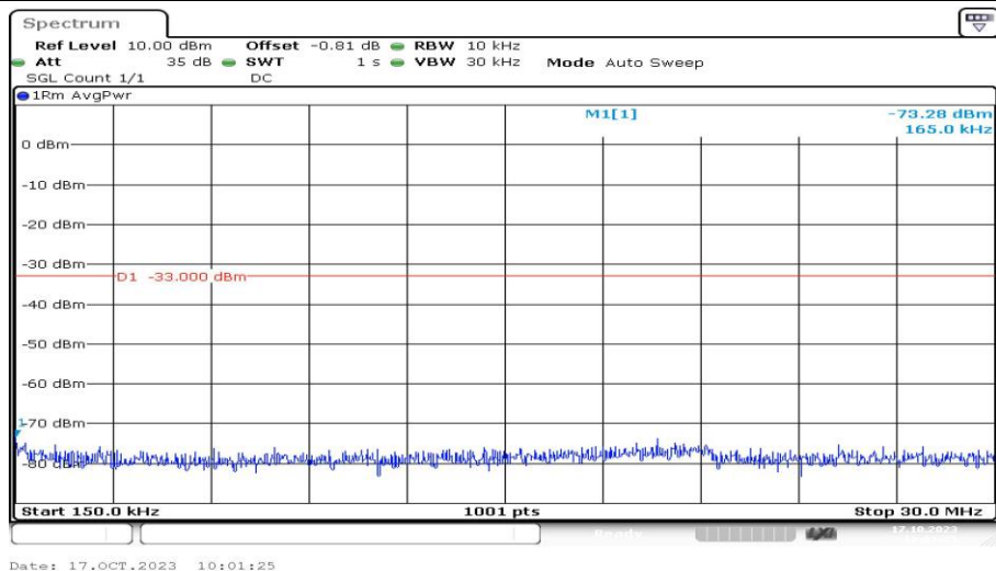
Band2-9538-1-0.15~30MHz-PASS
