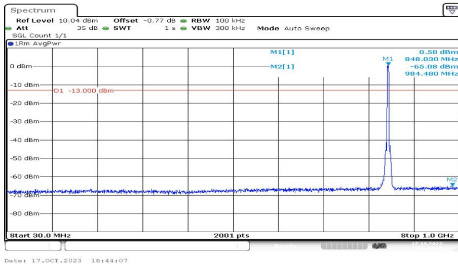
Band5-4233-1-30~1000MHz-PASS
