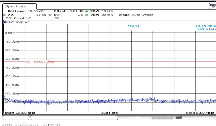
Band2-9400-2-0.15~30MHz-PASS
