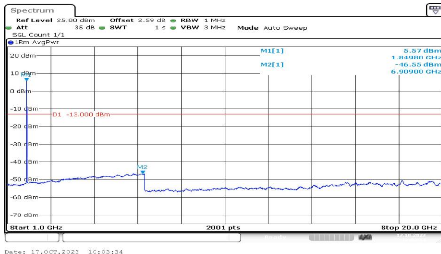
Band2-9262-2-1000~20000MHz-PASS
