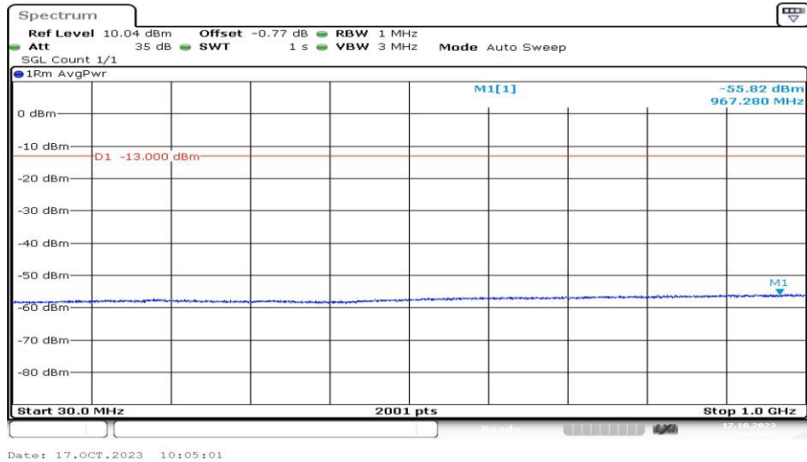
Band2-9400-2-30~1000MHz-PASS
