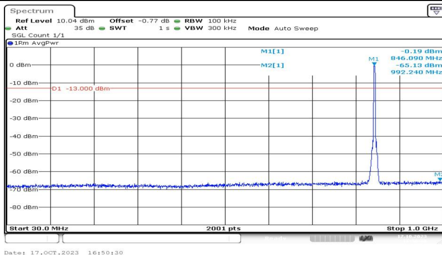
Band5-4233-3-30~1000MHz-PASS
