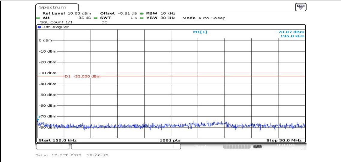
Band2-9538-2-0.15~30MHz-PASS
