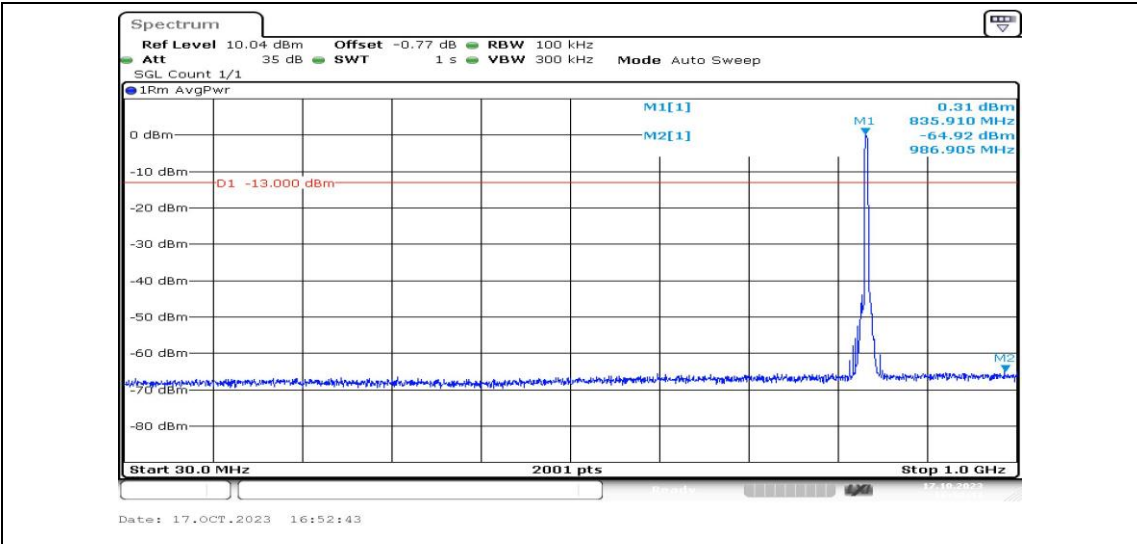
Band5-4182-4-30~1000MHz-PASS
