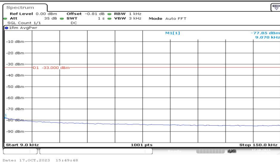
Band5-4233-0.009~0.15MHz-PASS
