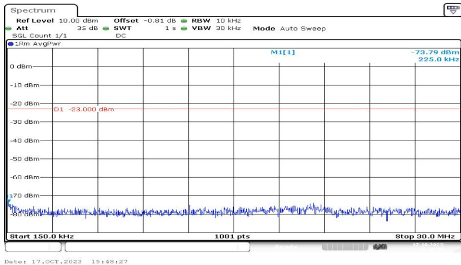
Band5-4132-0.15-30MHz-PASS
