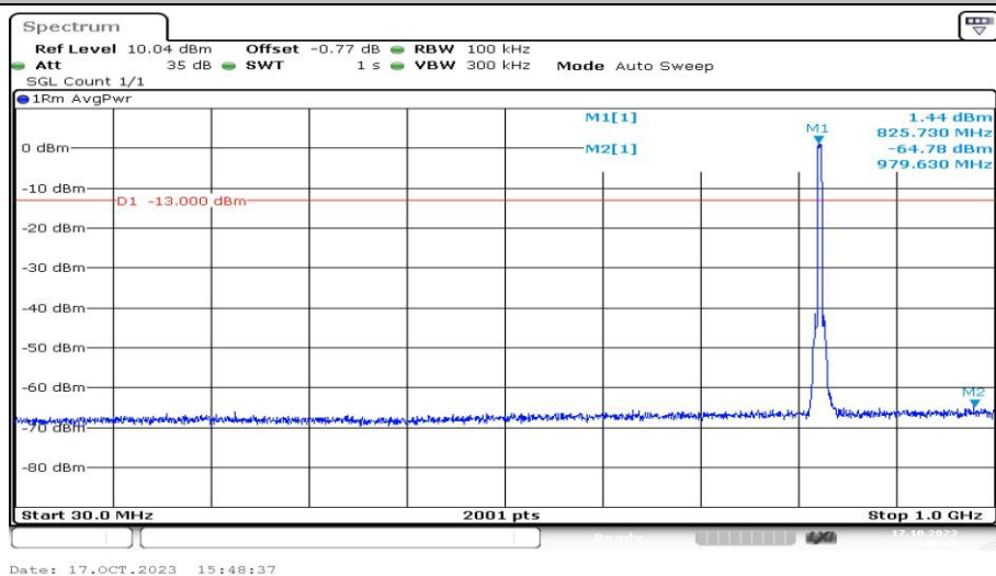
Band5-4132-30-1000MHz-PASS
