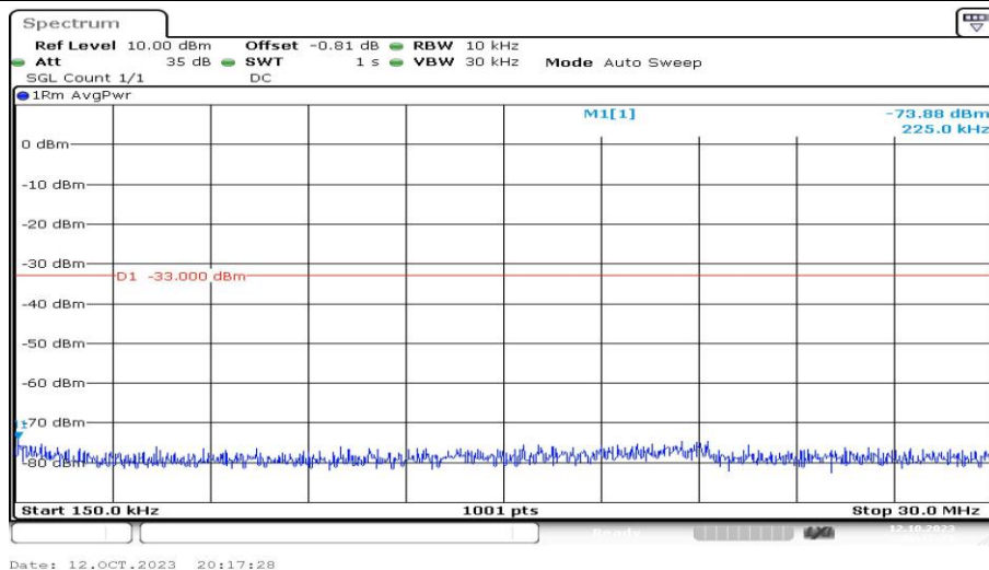
Band2-9538-1-0.15~30MHz-PASS
