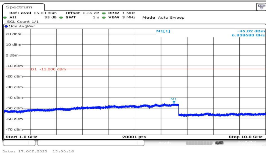
Band5-4233-1000~10000MHz-PASS
