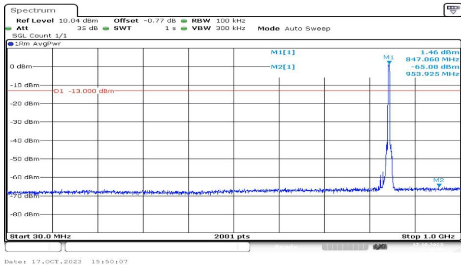
Band5-4233-30~1000MHz-PASS
