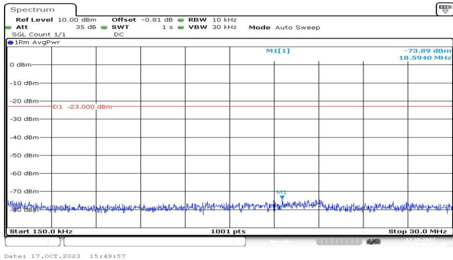
Band5-4233-0.15~30MHz-PASS
