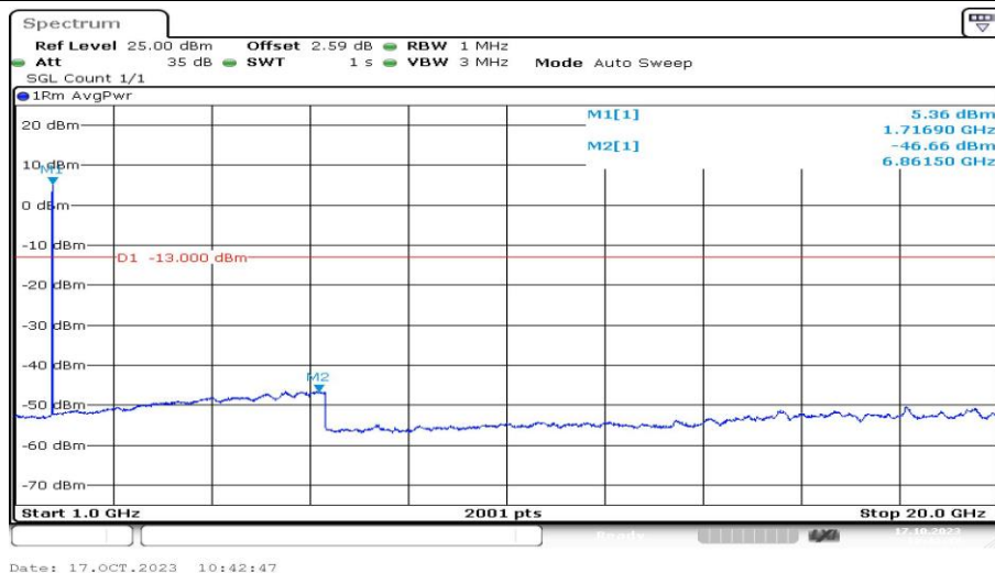
Band4-1312-1000~20000MHz-PASS
