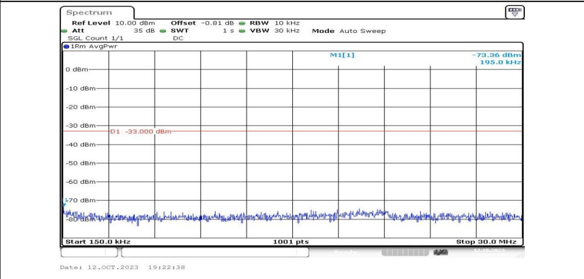
Band2-9262-0.15~30MHz-PASS
