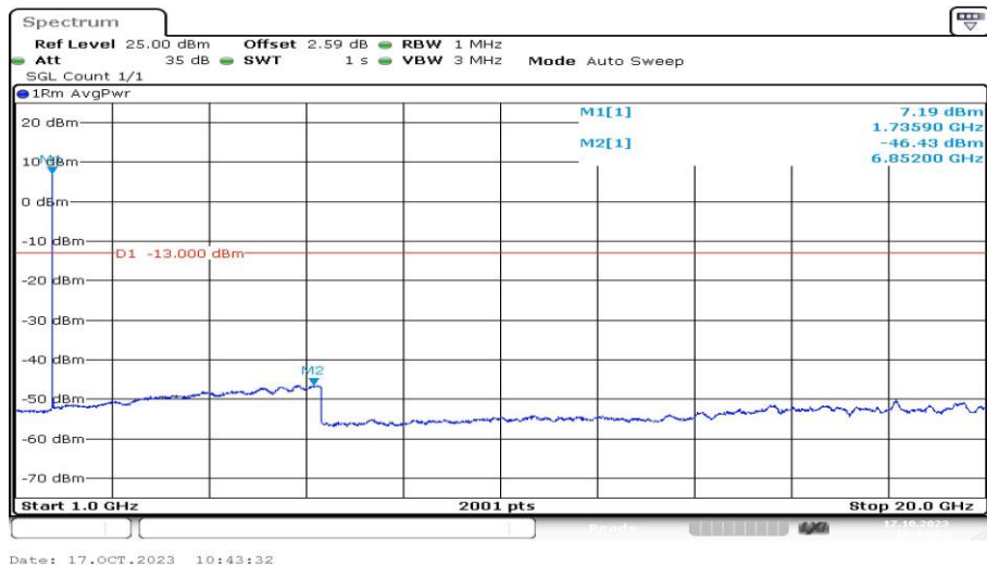
Band4-1413-1000~20000MHz-PASS
