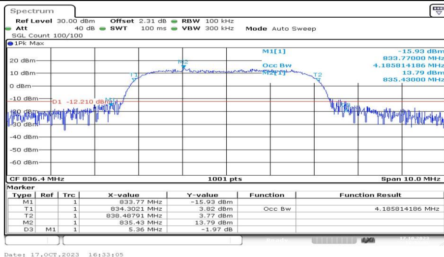
Band5-4182-2-PASS
