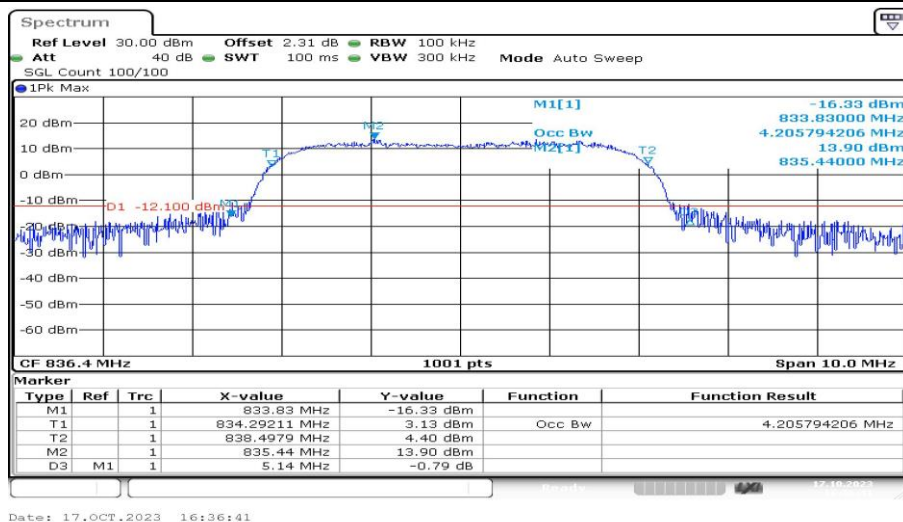
Band5-4182-4-PASS
