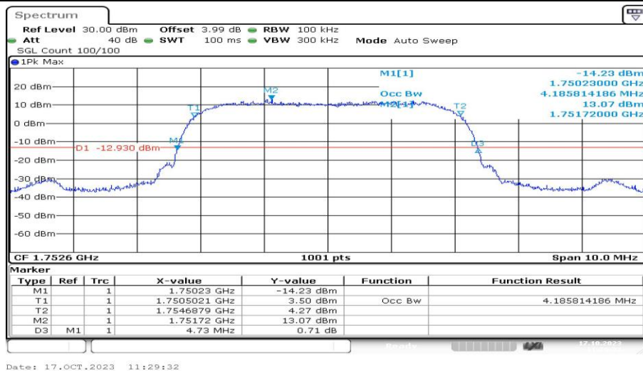
Band4-1513-3-PASS
