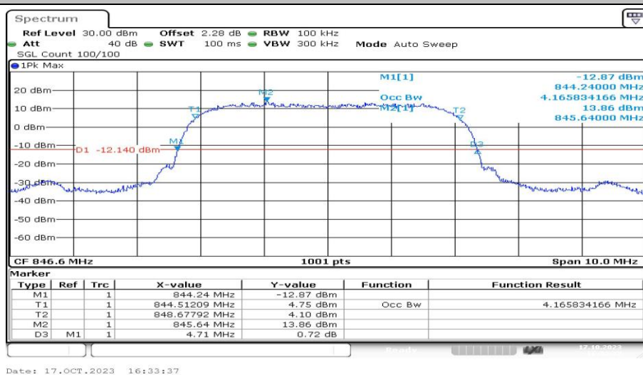
Band5-4233-2-PASS
