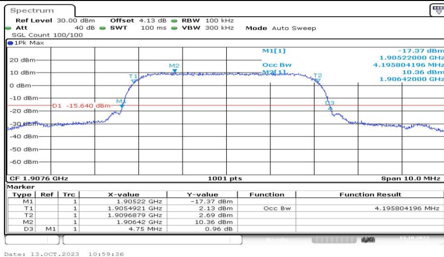
Band2-9538-4-PASS
