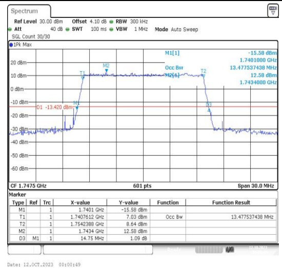
Band4-15MHz-16QAM-20325-75RB#0-PASS
