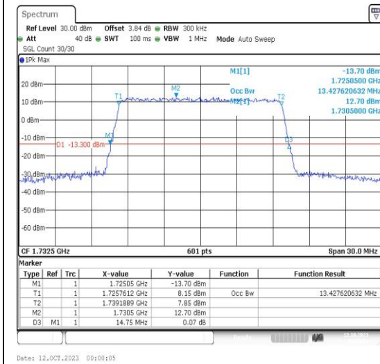
Band4-15MHz-QPSK-20175-75RB#0-PASS
