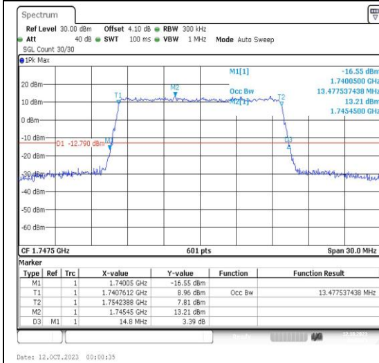
Band4-15MHz-QPSK-20325-75RB#0-PASS
