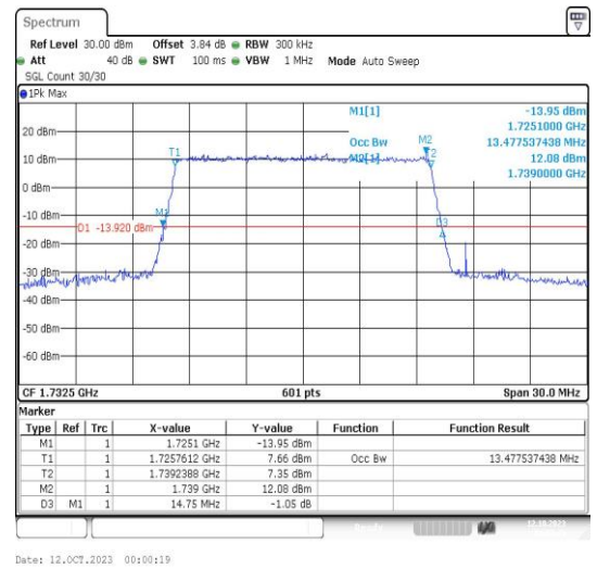
Band4-15MHz-16QAM-20175-75RB#0-PASS
