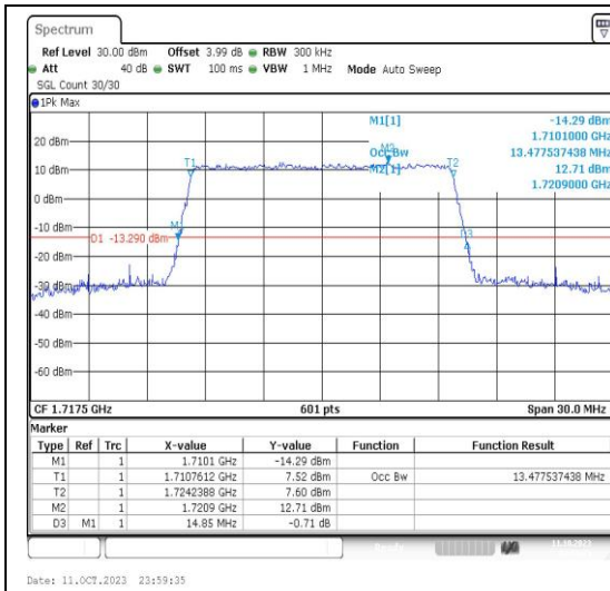
Band4-15MHz-QPSK-20025-75RB#0-PASS
