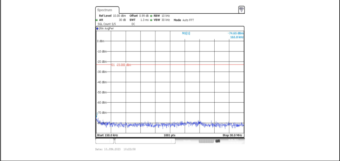
Band71-10MHz-16QAM-133297-1RB#0-Range2:0.15~30MHz
