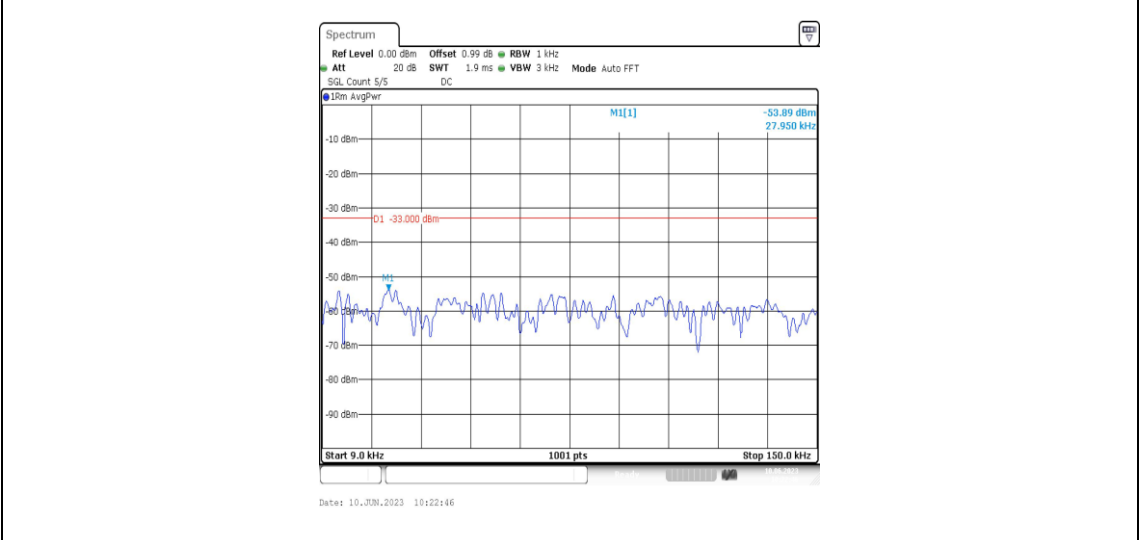
Band71-10MHz-16QAM-133297-1RB#0-Range1:0.009~0.15MHz
