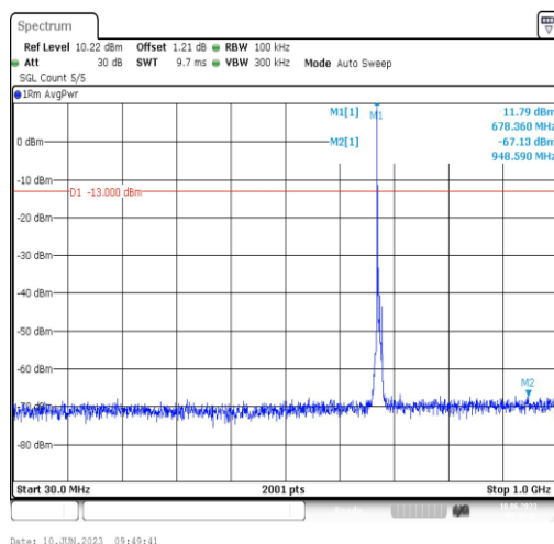
Band71-5MHz-16QAM-133297-1RB#0-Range3:30~1000MHz
