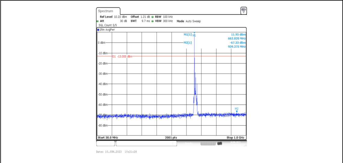
Band71-10MHz-16QAM-133172-1RB#0-Range3:30~1000MHz
