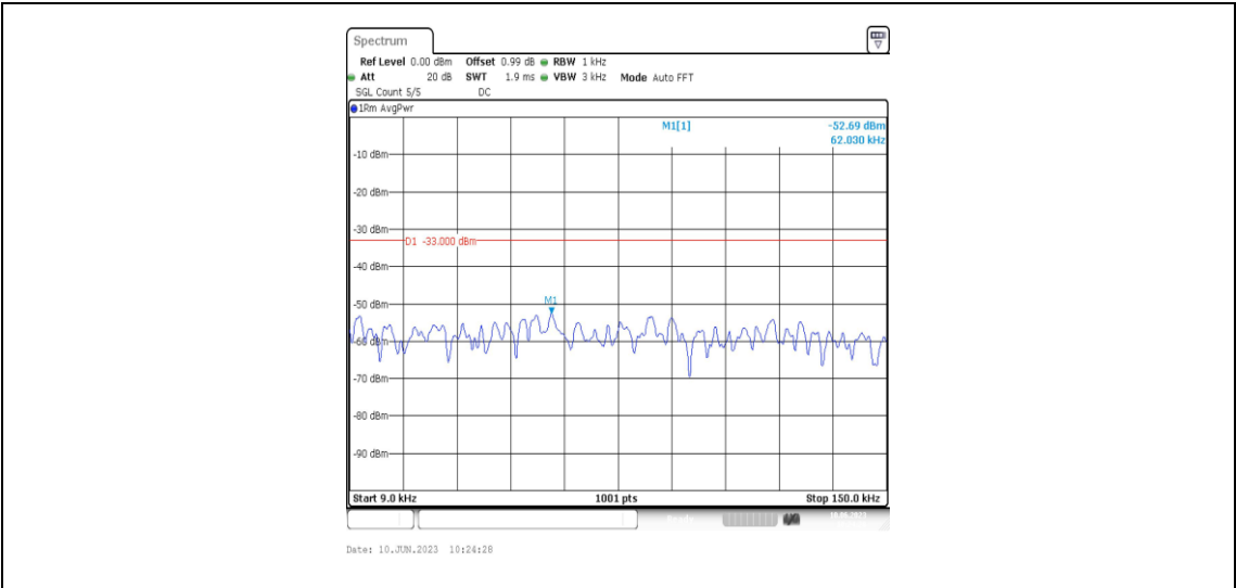
Band71-10MHz-16QAM-133422-1RB#0-Range1:0.009~0.15MHz
