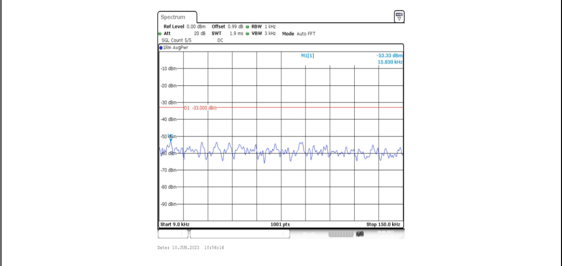
Band71-15MHz-16QAM-133297-1RB#0-Range1:0.009~0.15MHz
