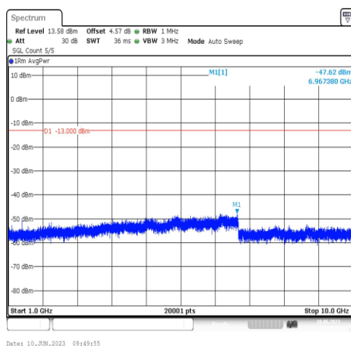
Band71-5MHz-16QAM-133297-1RB#0-Range4:1000~10000MHz
