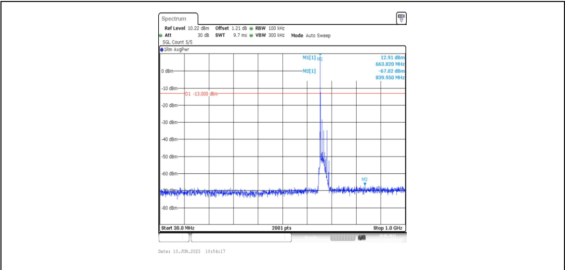
Band71-15MHz-QPSK-133197-1RB#0-Range3:30~1000MHz
