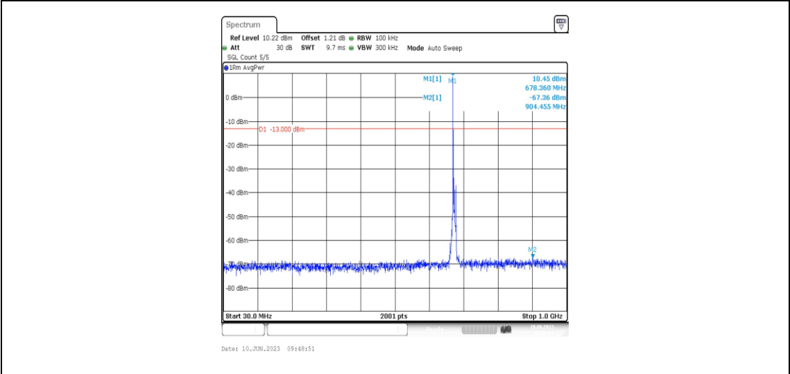
Band71-5MHz-QPSK-133297-1RB#0-Range3:30~1000MHz
