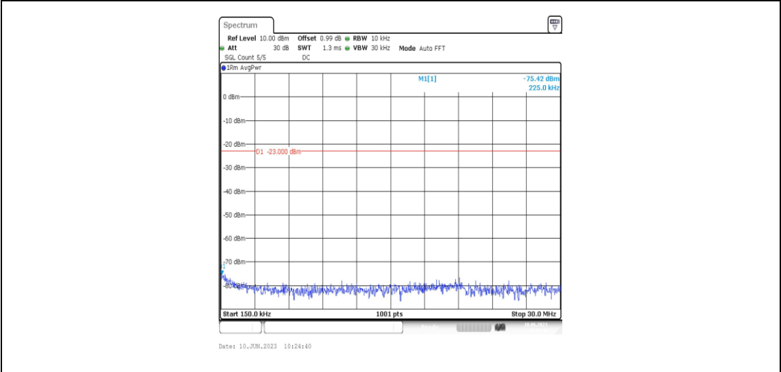
Band71-10MHz-16QAM-133422-1RB#0-Range2:0.15~30MHz
