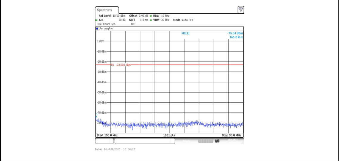
Band71-15MHz-16QAM-133297-1RB#0-Range2:0.15~30MHz
