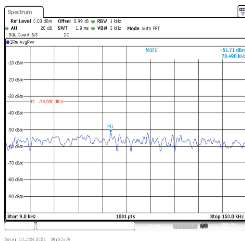
Band71-5MHz-QPSK-133447-1RB#0-Range1:0.009~0.15MHz
